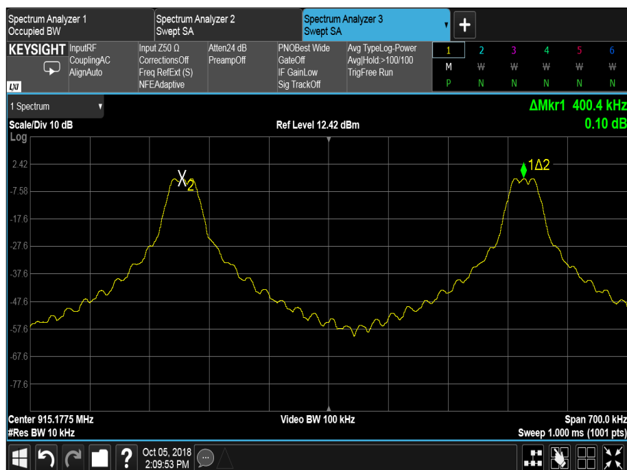
Figure 5 - GFSK
