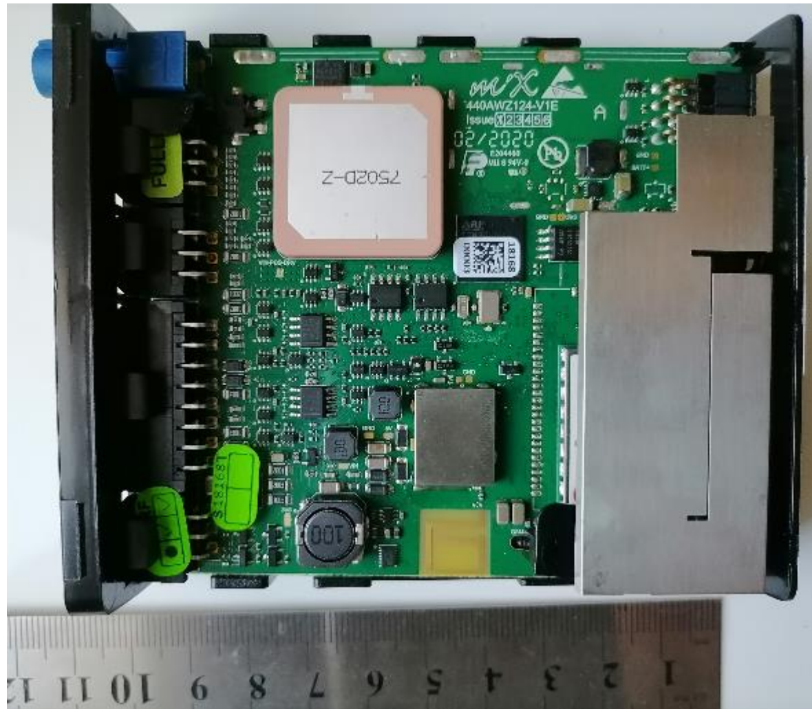
Figure 4: View of PCB (top view)
