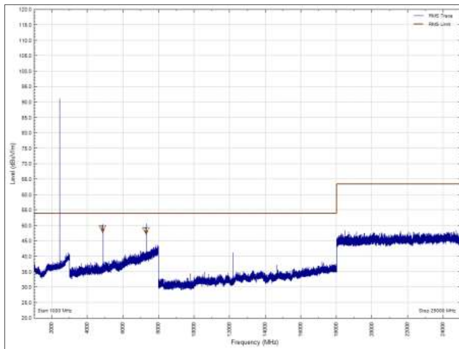
Figure 30 - 2440 MHz - 1 GHz to 25 GHz, Vertical, EUT Orientation: X, Average
