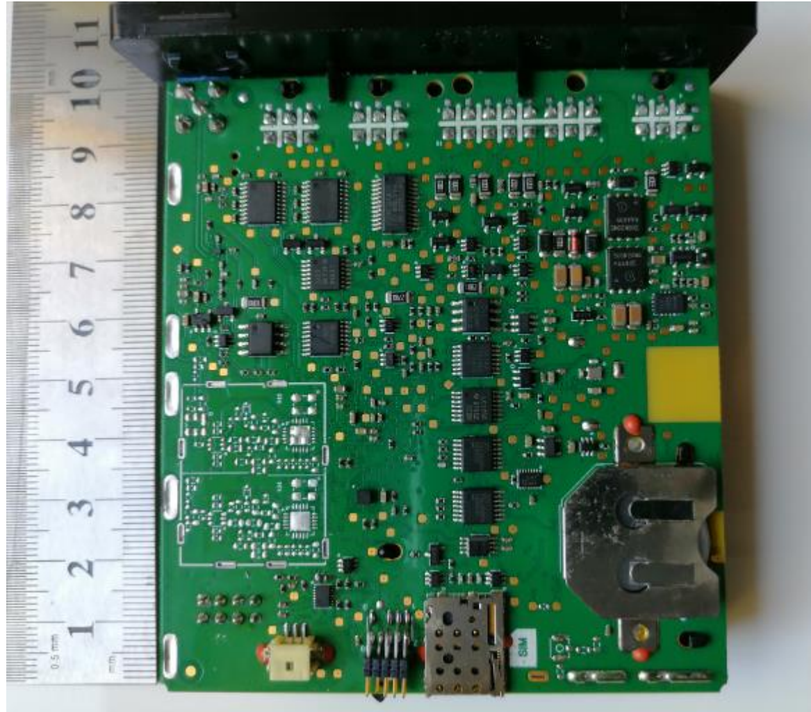
Figure 7: Bottom side of Main PCB
