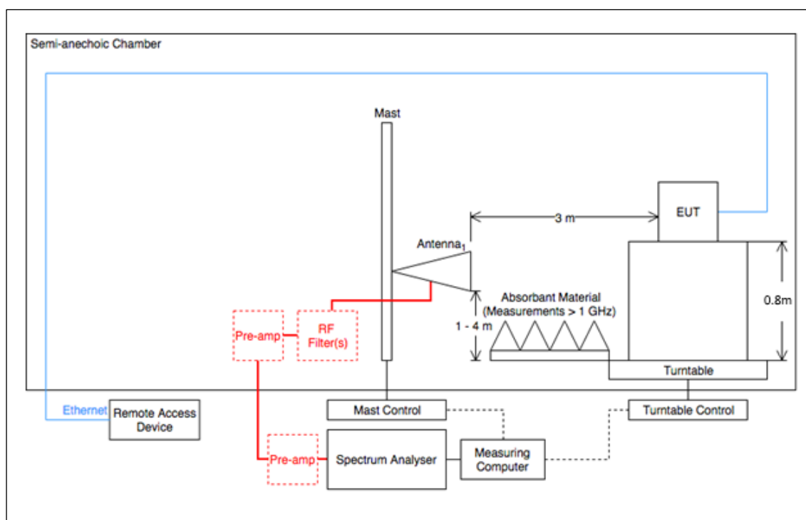
Figure 4 - Radiated Disturbance Example Test Setup
