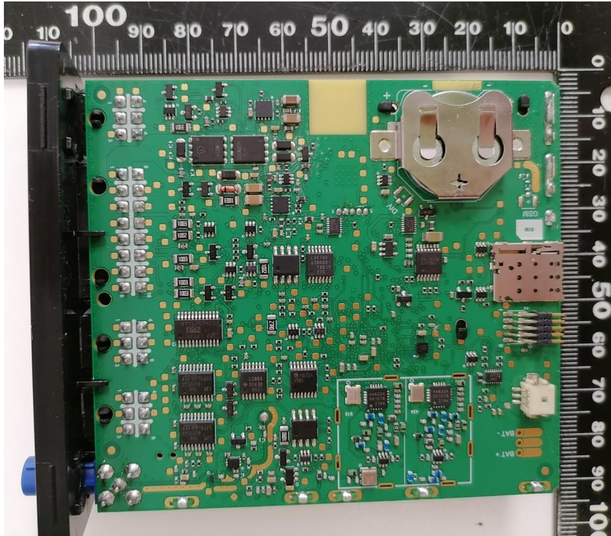
Figure 9: Bottom Side of PCB (MiX 4401-B with SRD 434/915MHz circuits populated)
