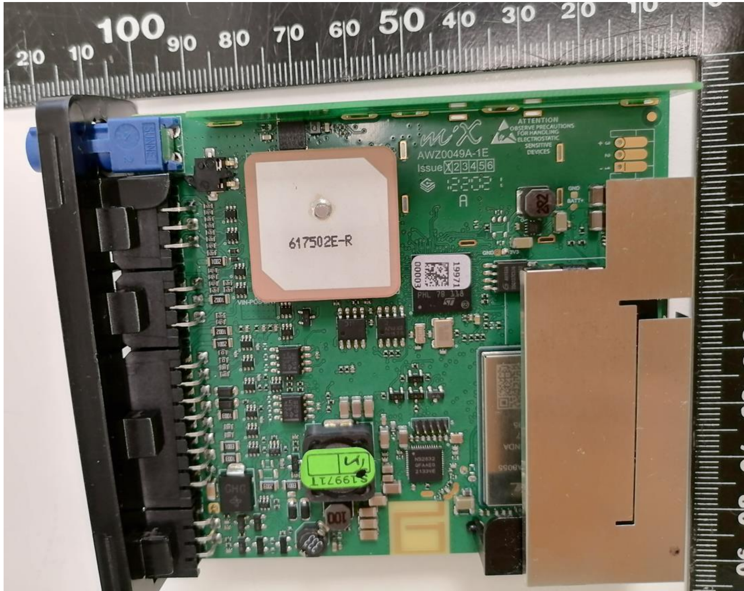
Figure 4: View of PCB (top view) (with modem antenna)
