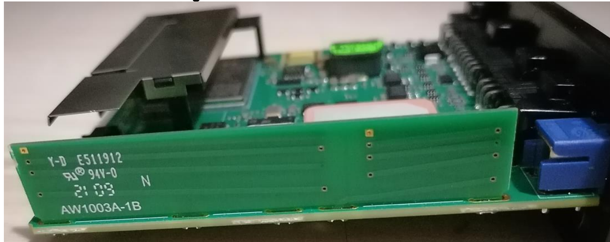
Figure 6: Side View of SRD Antenna (AW1003A-1B)
