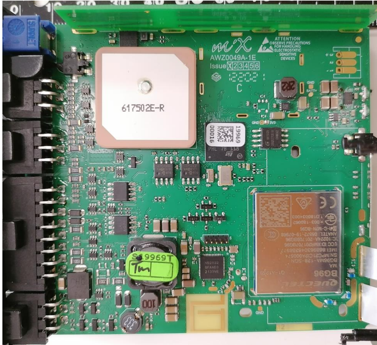
Figure 7: View of MiX 4401/-B Main PCB – without modem antenna (BG96 modem)
