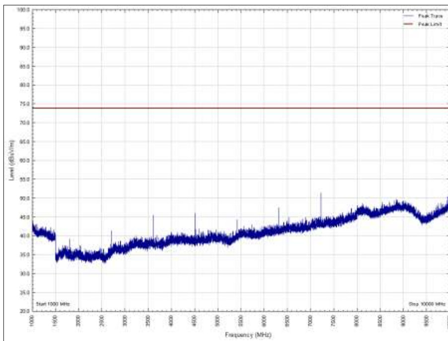
Figure 14 - 902.2 MHz, 1 GHz to 10 GHz, Vertical, X Orientation: - Peak
