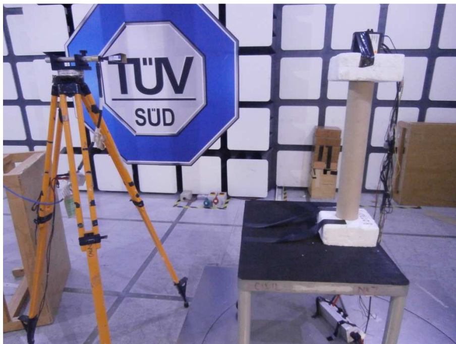
FCC Part 15.407 Radiated Emissions 18 GHz to 25 GHz
