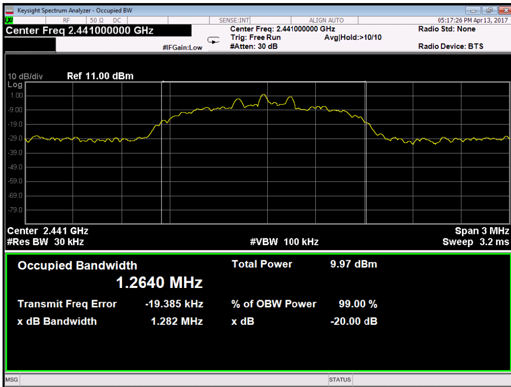
39 Channel @ 8-DPSK
