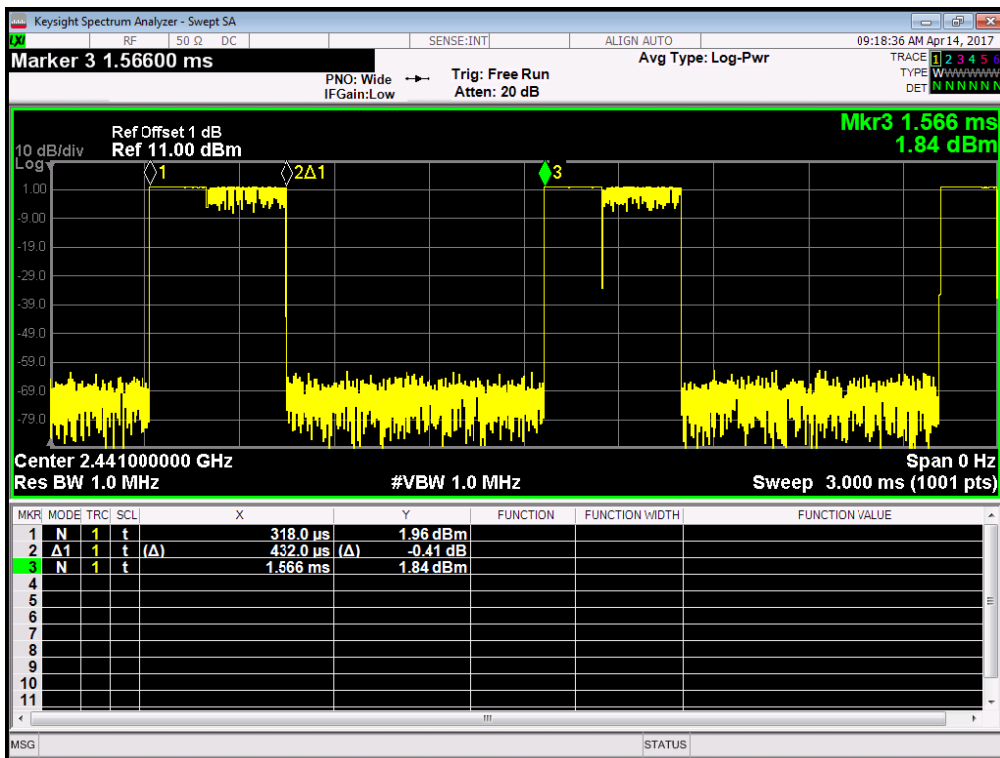
39 Channel @ 2DH1
