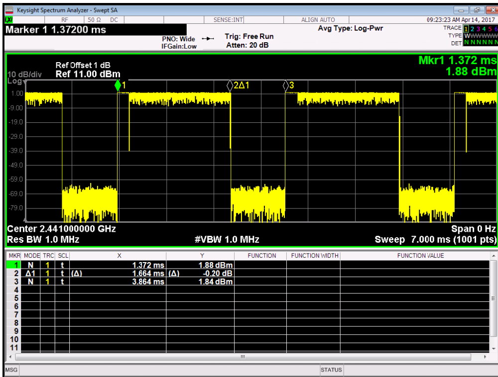
39 Channel @ 2DH3
