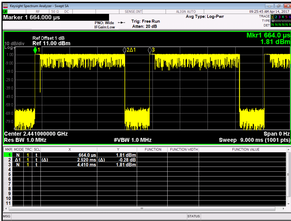
39 Channel @ DH5
