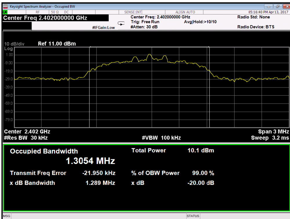
0 Channel @ 8-DPSK
