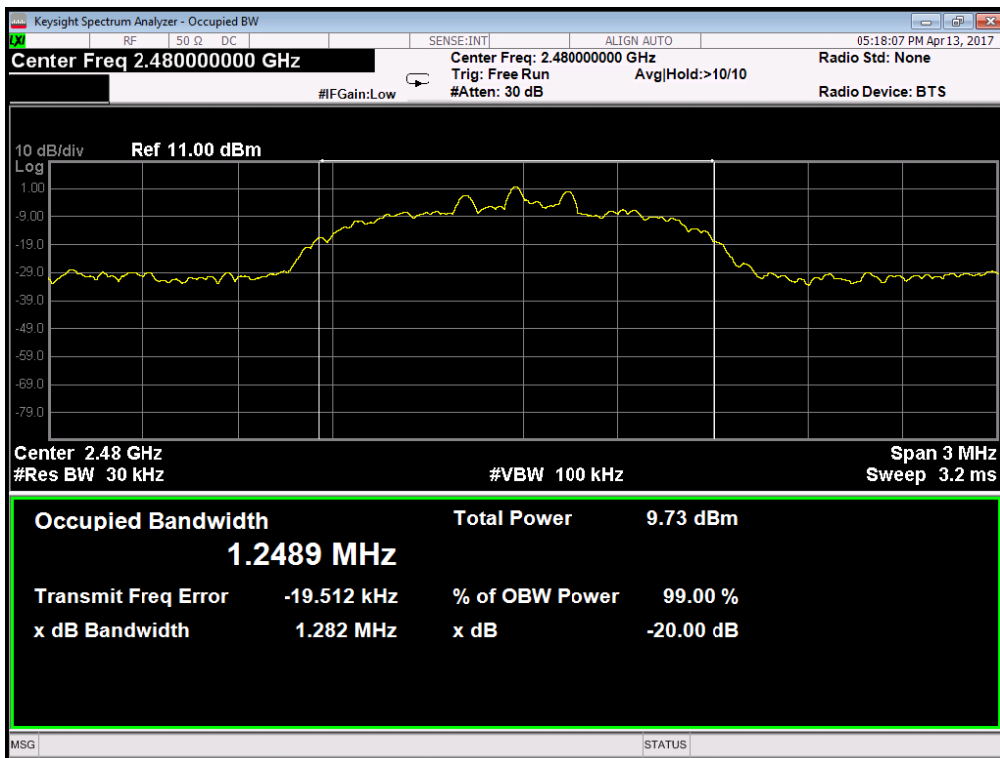
78 Channel @ 8-DPSK
