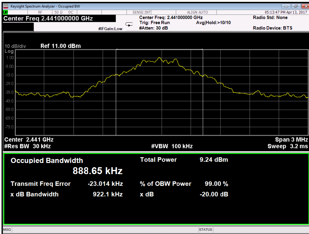
39 Channel @ GFSK
