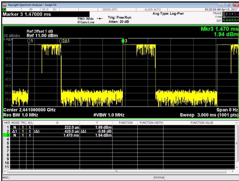
39 Channel @ 3DH1
