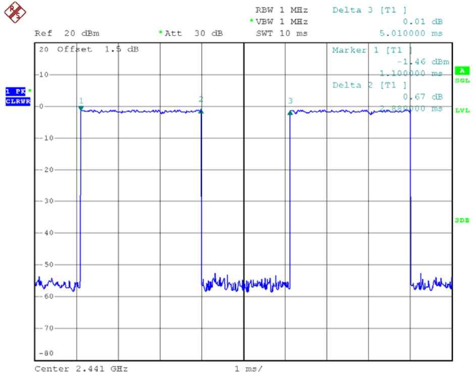
39 Channel @ 3DH5
