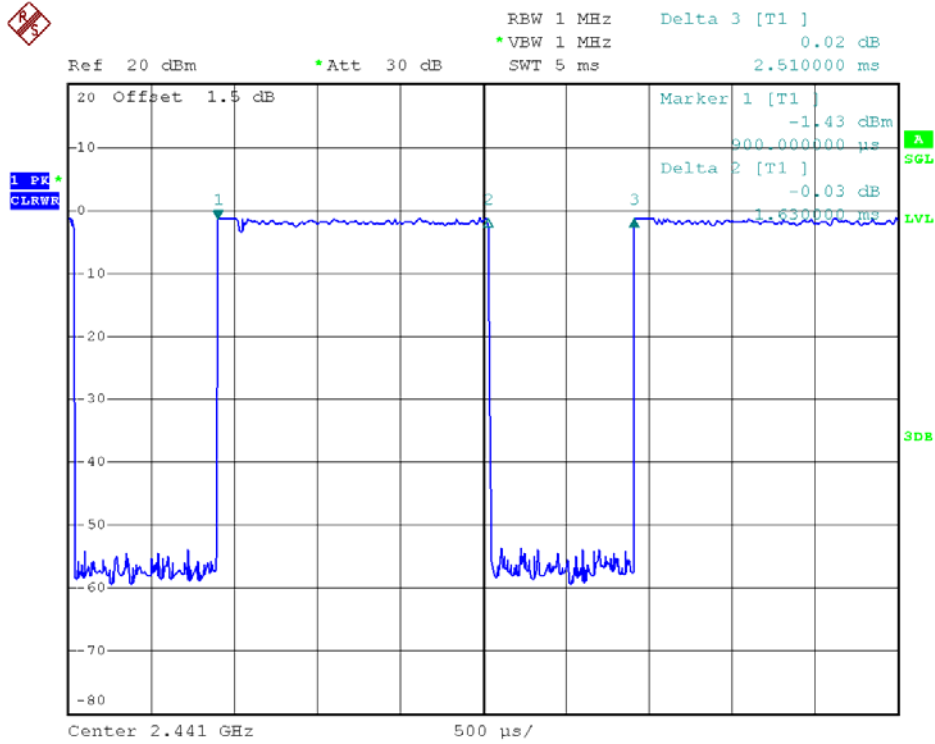
39 Channel @ 2DH3
