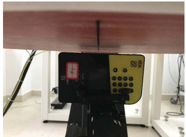
Body-worn Right Side (5mm)
