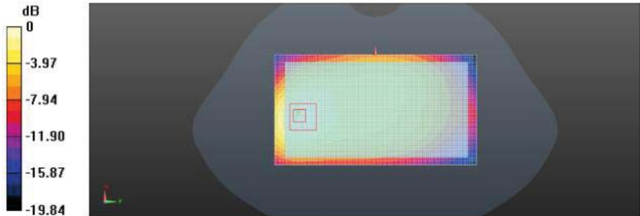
Rear Side (GSM850 GPRS 2TS Middle Channel)
