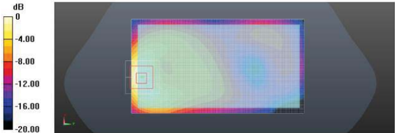
Rear Side (PCS1900 GPRS 2TS Middle Channel)
