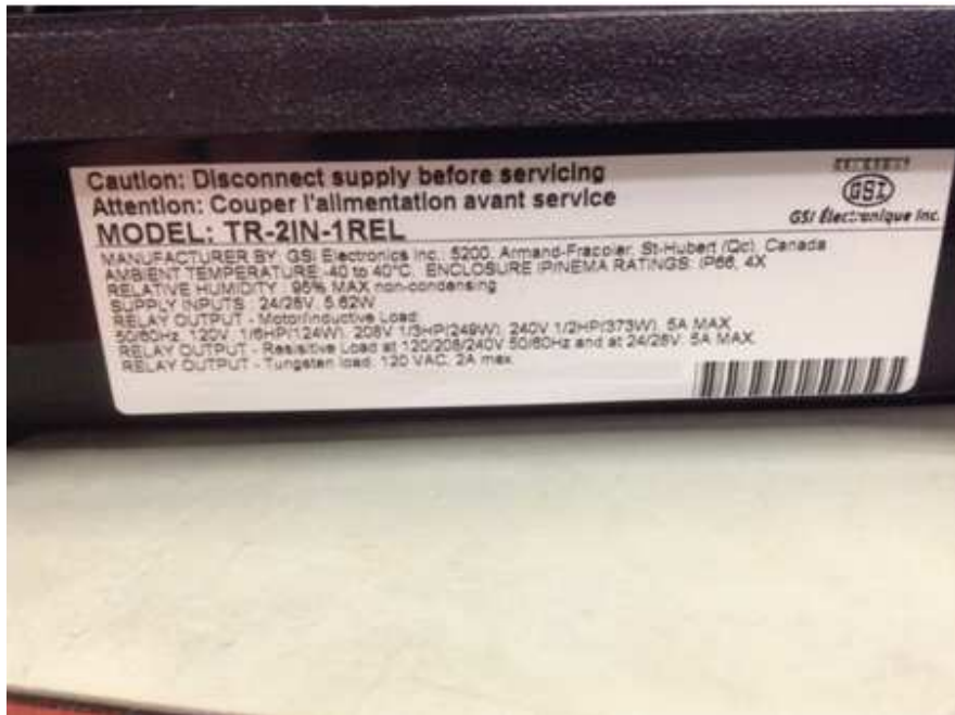
Side view of TR-2IN-1REL
