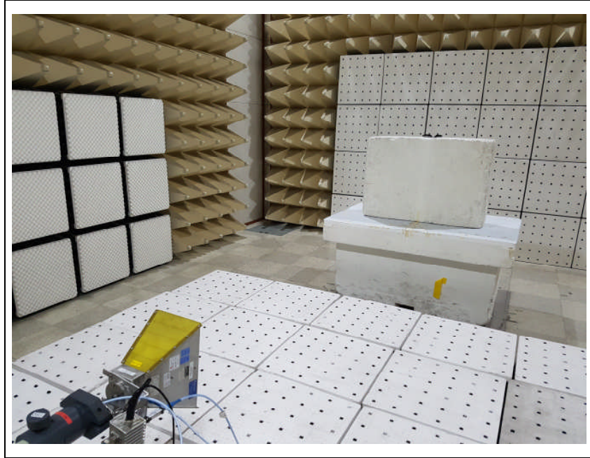
- Photo of Radiated Spurious Emission Test (Above 1 GHz)
