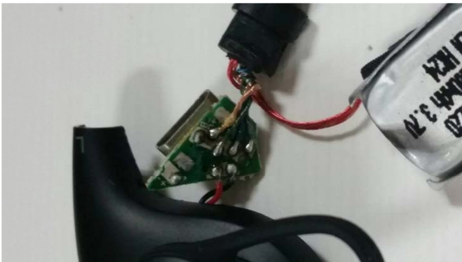
View of micro USB Board (Bottom)
