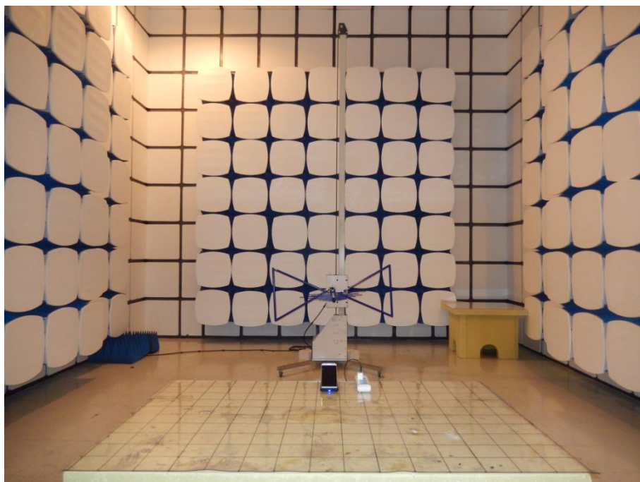
Radiated emission Measurement Photos(30MHz-1000MHz)
