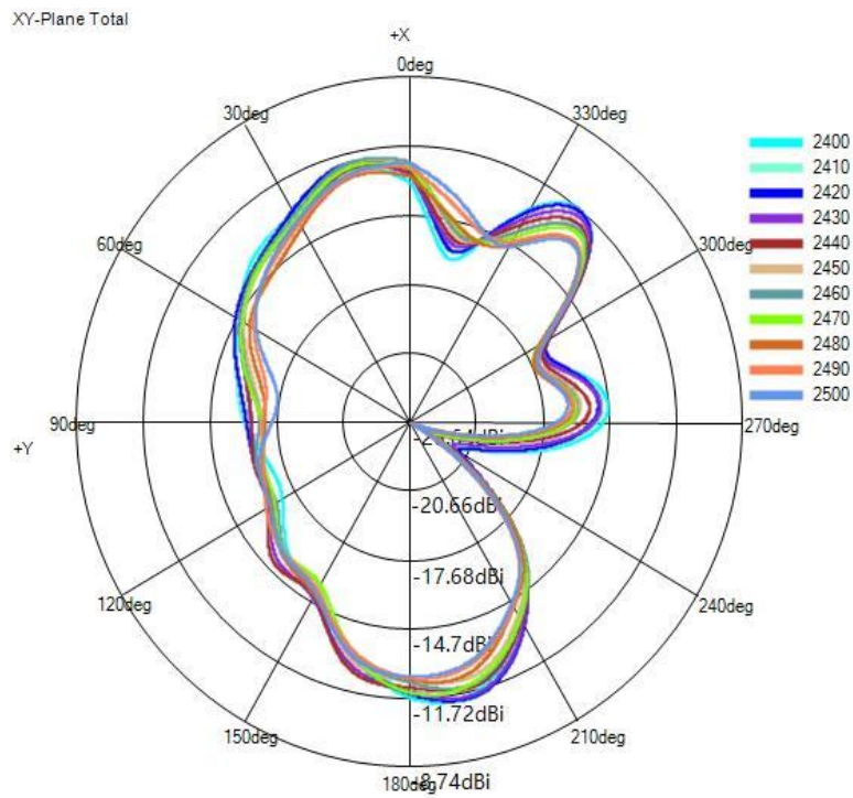
(3) X-Y Plane(unit:dBi):
