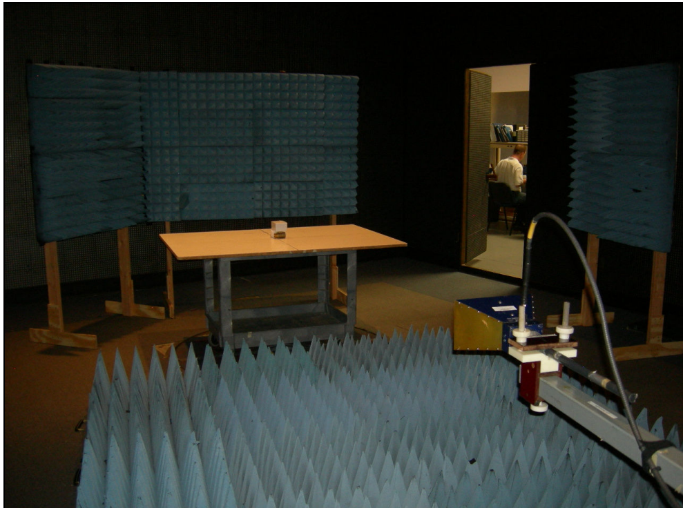
Figure 3: Radiated Emissions
