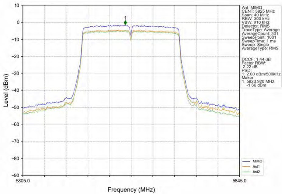
802.11ax(HEW20)_HCH_5825MHz_MIMO_NTNV
