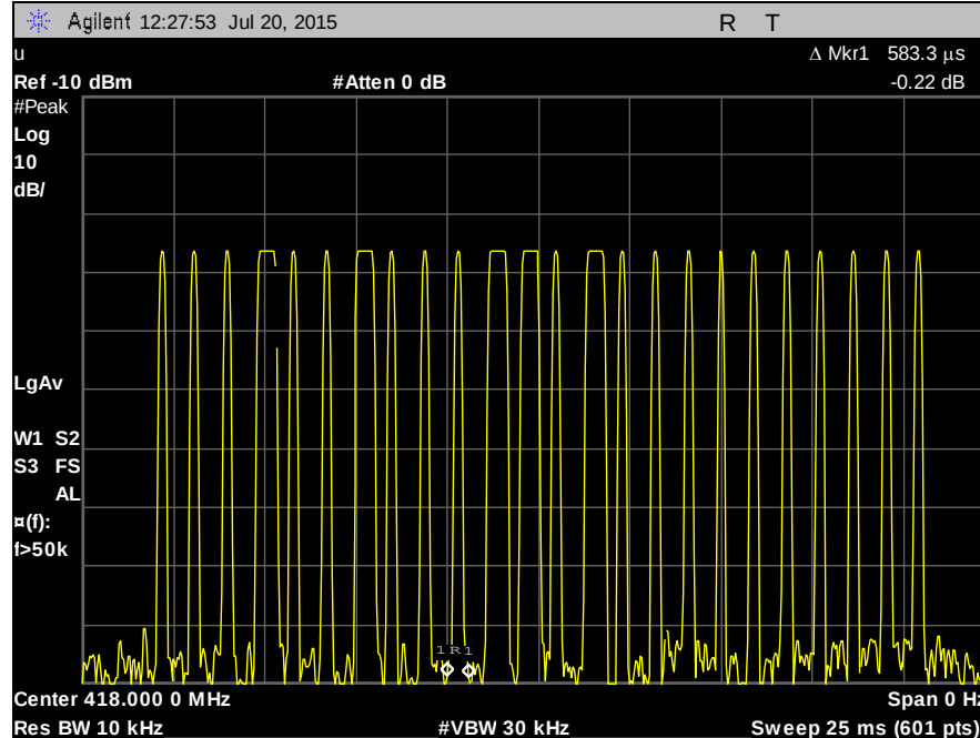
Plot 2. Duty Cycle, 25 ms Sweep, On Time, Narrow Pulse
