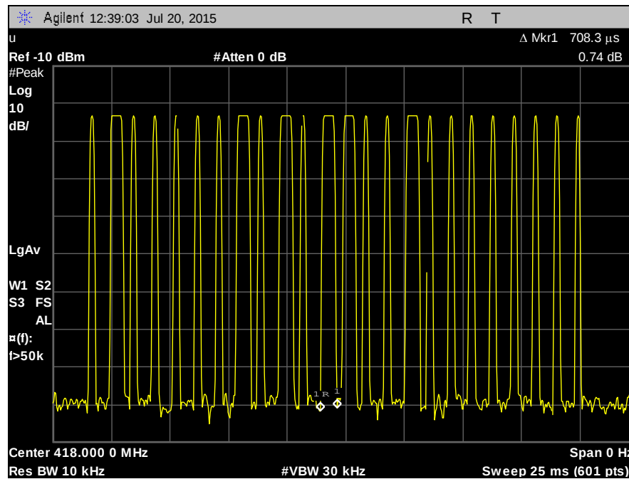
Plot 3. Duty Cycle, 25 ms Sweep, On Time, Wide Pulse
