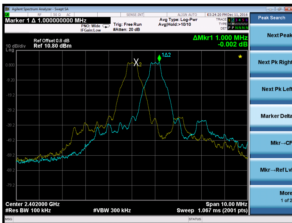
Figure 49: Frequency Separation, DH5, 2402MHz
