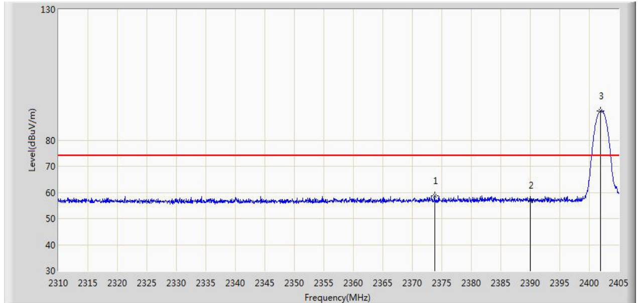
Figure 43: Band Edge, 3-DH5, 2402MHz, Vertical, PK
