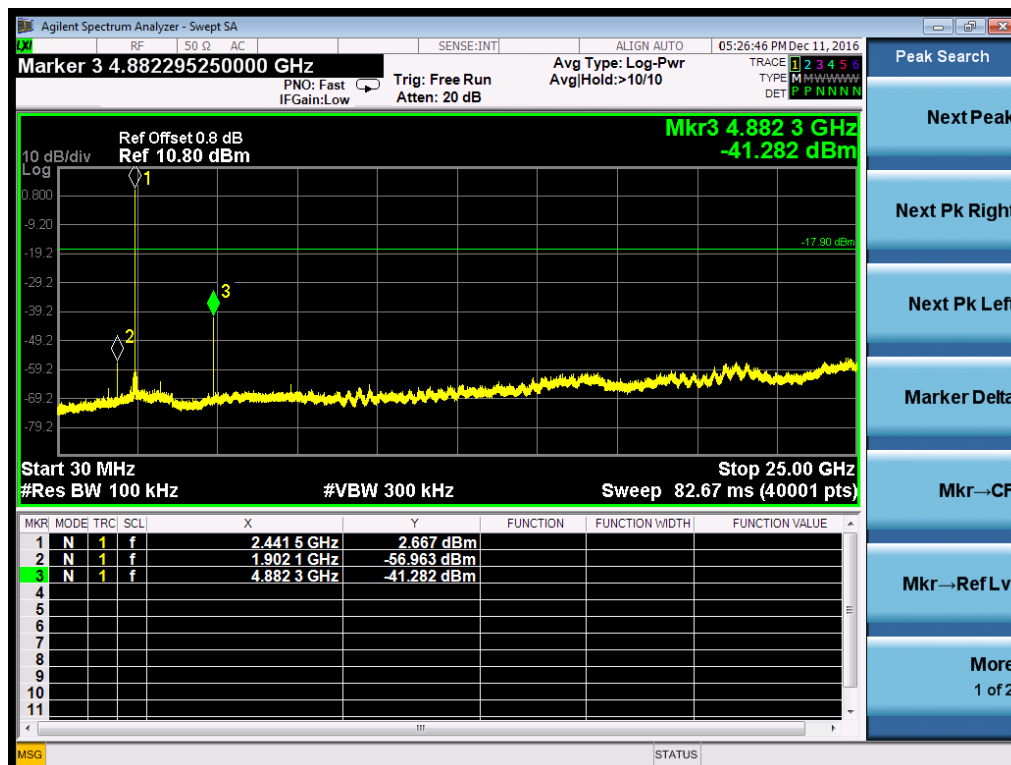
Figure 11: Conducted Spurious Emission, DH5, 2441MHz
