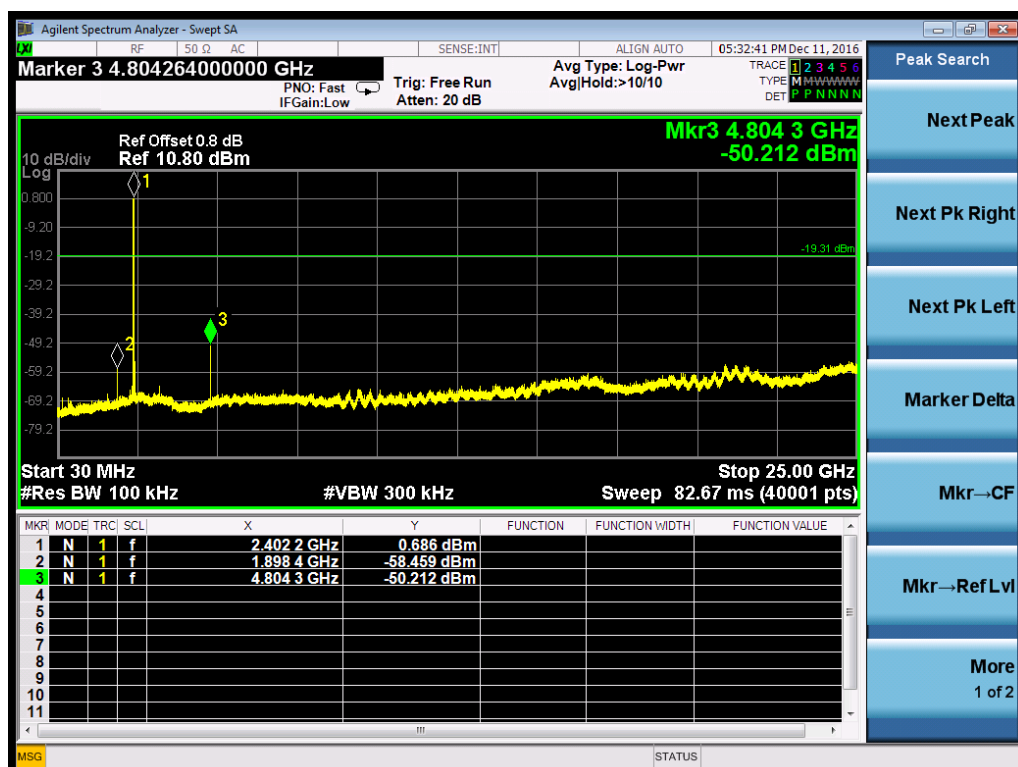
Figure 13: Conducted Spurious Emission, 2-DH5, 2402MHz
