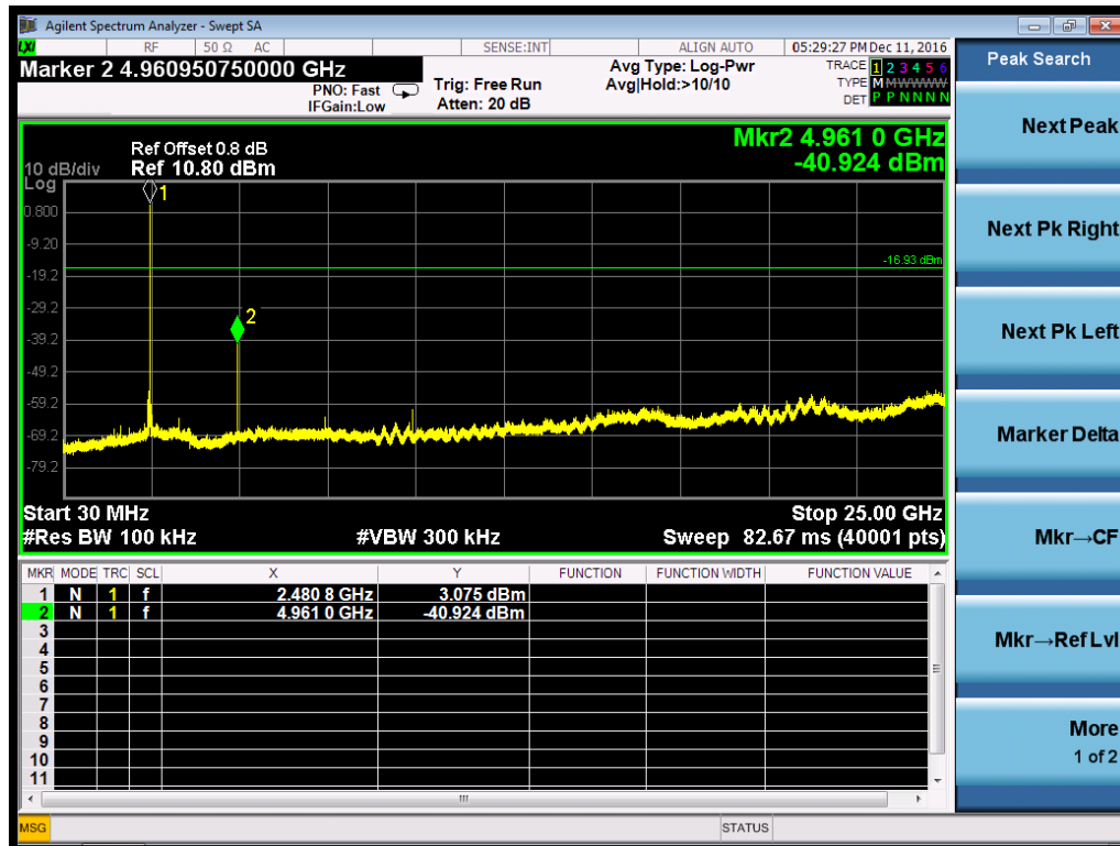
Figure 12: Conducted Spurious Emission, DH5, 2480MHz
