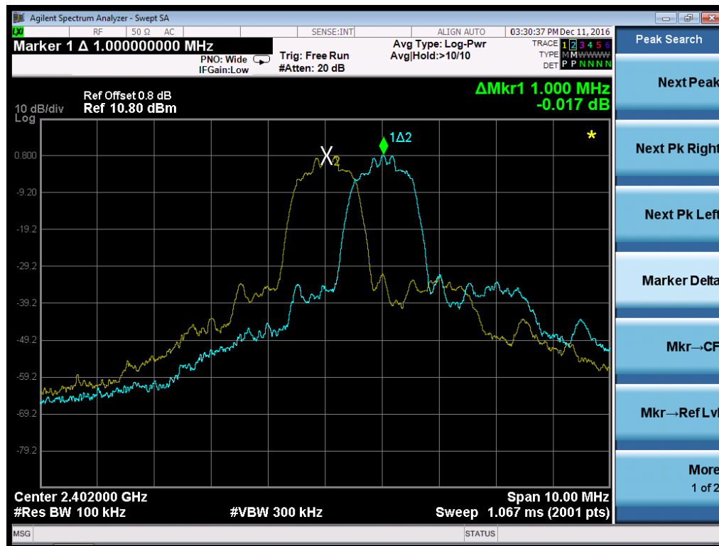
Figure 52: Frequency Separation, 2-DH5, 2402MHz
