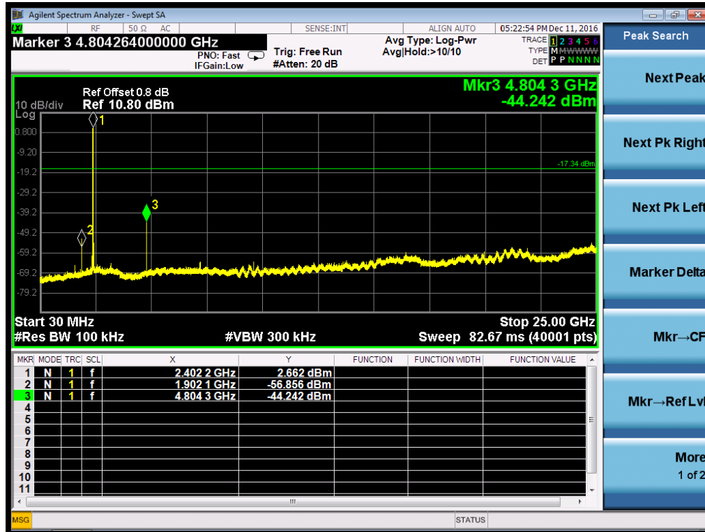
Figure 10: Conducted Spurious Emission, DH5, 2402MHz
