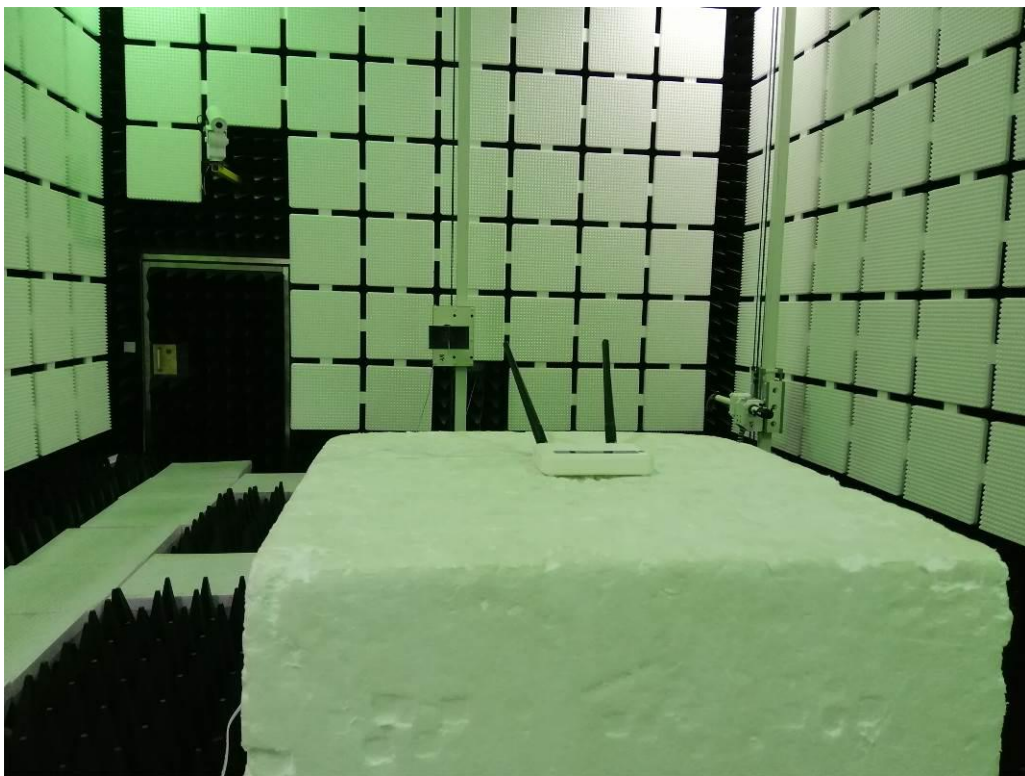
Fig. 4(MSA-C1500IC12.0-18P-zz)
