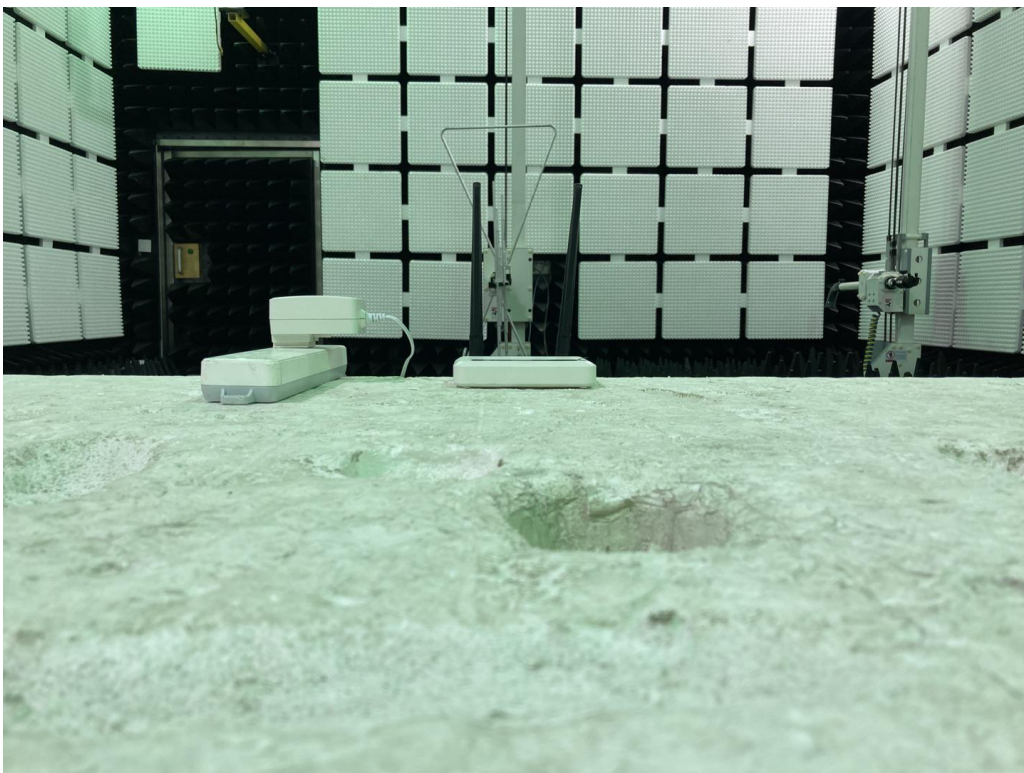
Fig. 2(MSA-C1500IC12.0-18P-zz)
