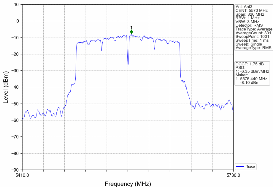
802.11ac(VHT160)_MCH_5570MHz_Ant3_NTNV
