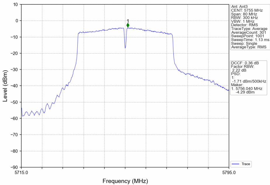
802.11ac(VHT40)_LCH_5755MHz_Ant3_NTNV
