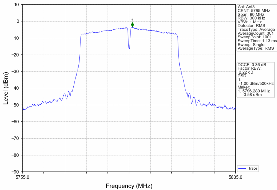
802.11ac(VHT40)_HCH_5795MHz_Ant3_NTNV
