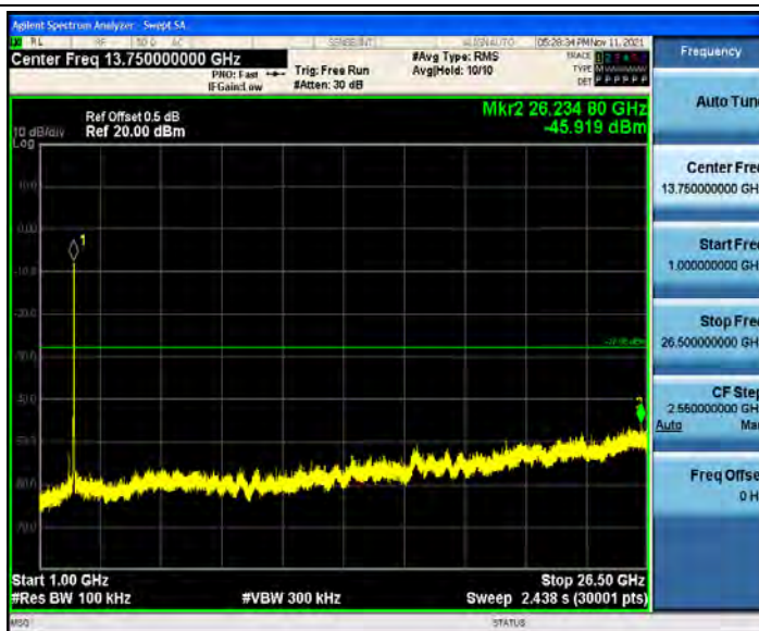
802.11n(HT40)_Ant2_2437_0~Reference
