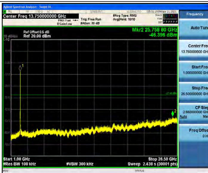
802.11n(HT40)_Ant1_2452_0~Reference
