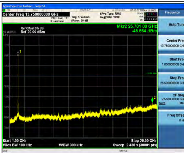
802.11n(HT40)_Ant1_2422_0~Reference
