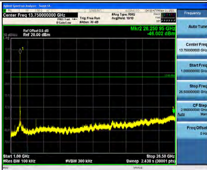
802.11g_Ant1_2412_0~Reference
