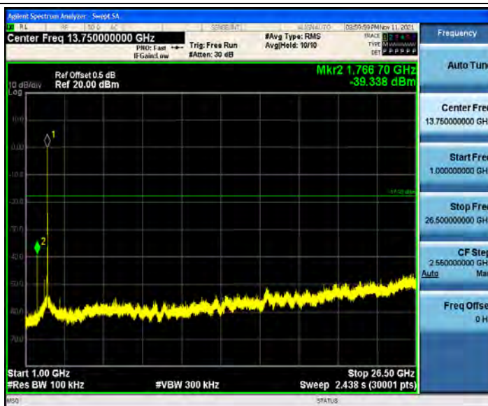
802.11g_Ant2_2437_0~Reference
