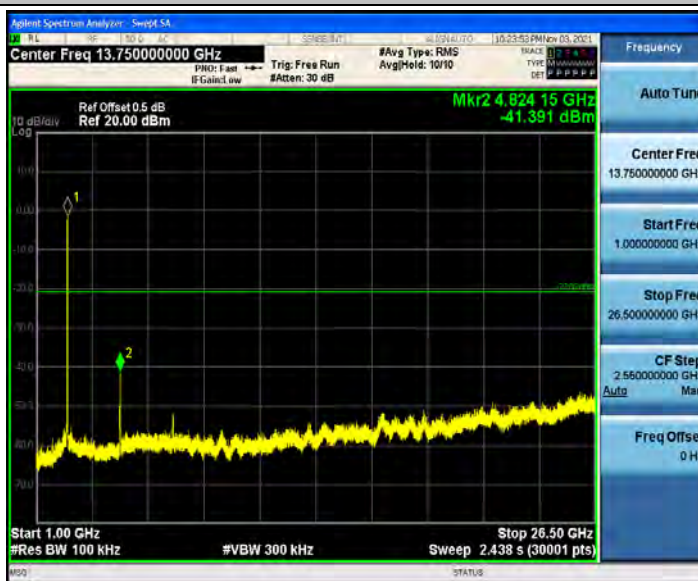
802.11n(HT20)_Ant1_2437_0~Reference
