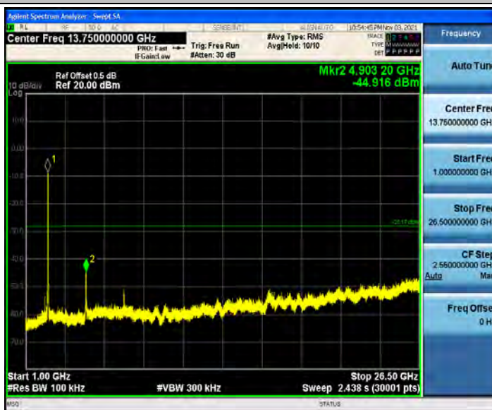
802.11n(HT40)_Ant2_2452_0~Reference
