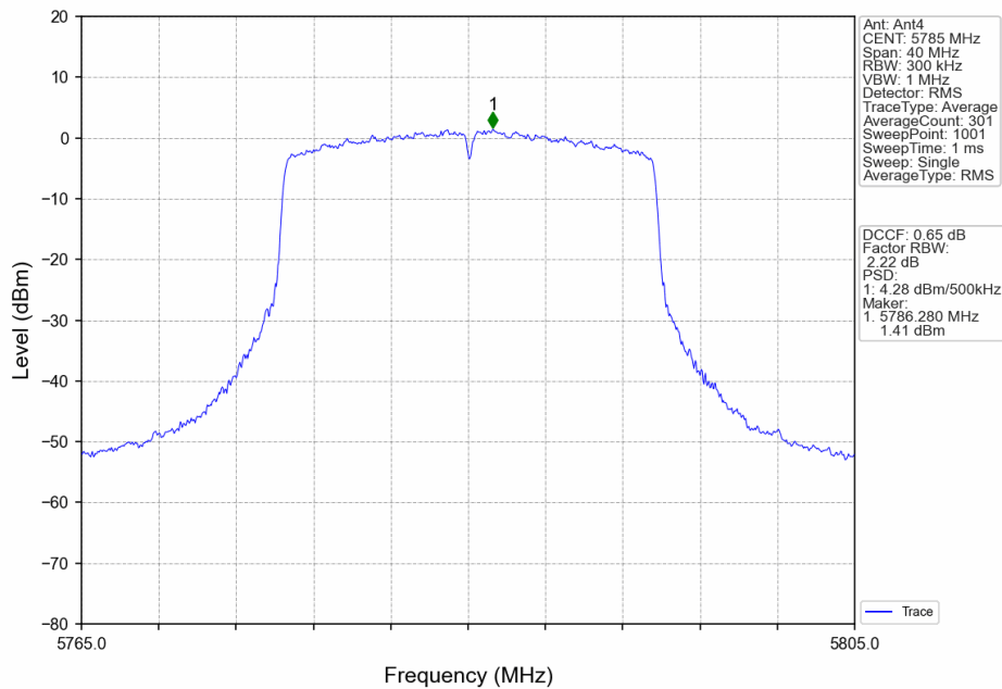
802.11ax(HEW20)_MCH_5785MHz_RU242_Left_Ant4_NTNV
