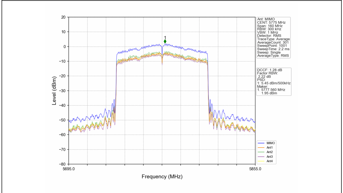
802.11ax(HEW80)_MCH_5775MHz_RU996_Left_MIMO_NTNV
