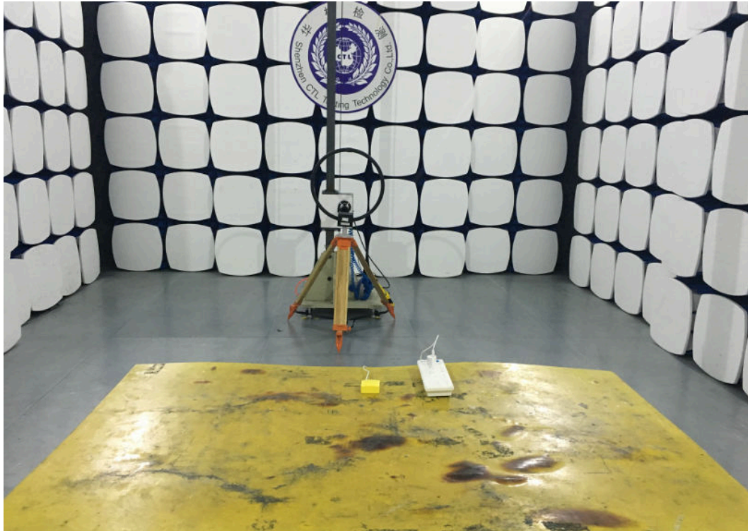
Radiated emission below 30MHz
