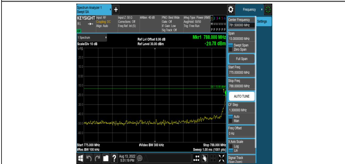
Band14-5MHz-QPSK-23305-1RB#0-Range7:775~788MHz
