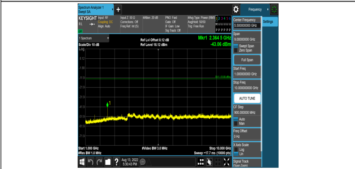
Band14-5MHz-QPSK-23305-1RB#0-Range4:1000~10000MHz
