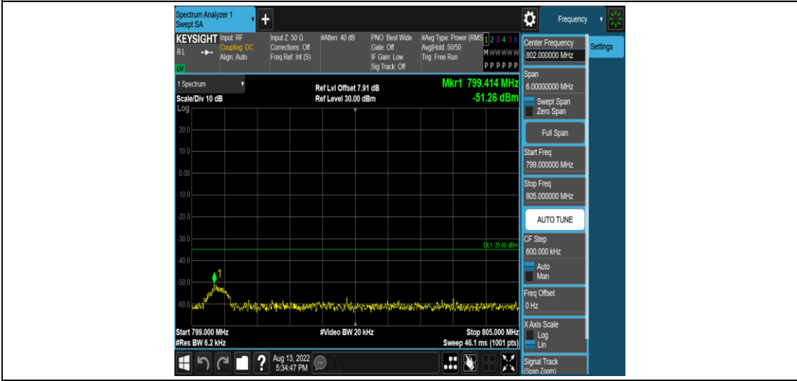
Band14-5MHz-QPSK-23330-1RB#0-Range6:799~805MHz
