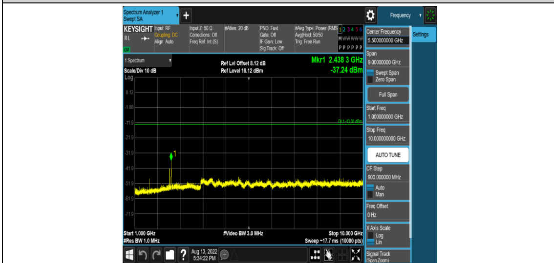
Band14-5MHz-QPSK-23330-1RB#0-Range4:1000~10000MHz
