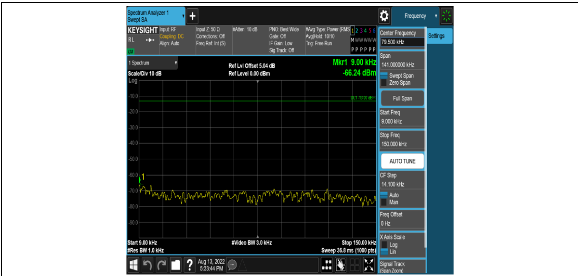
Band14-5MHz-QPSK-23330-1RB#0-Range1:0.009~0.15MHz
