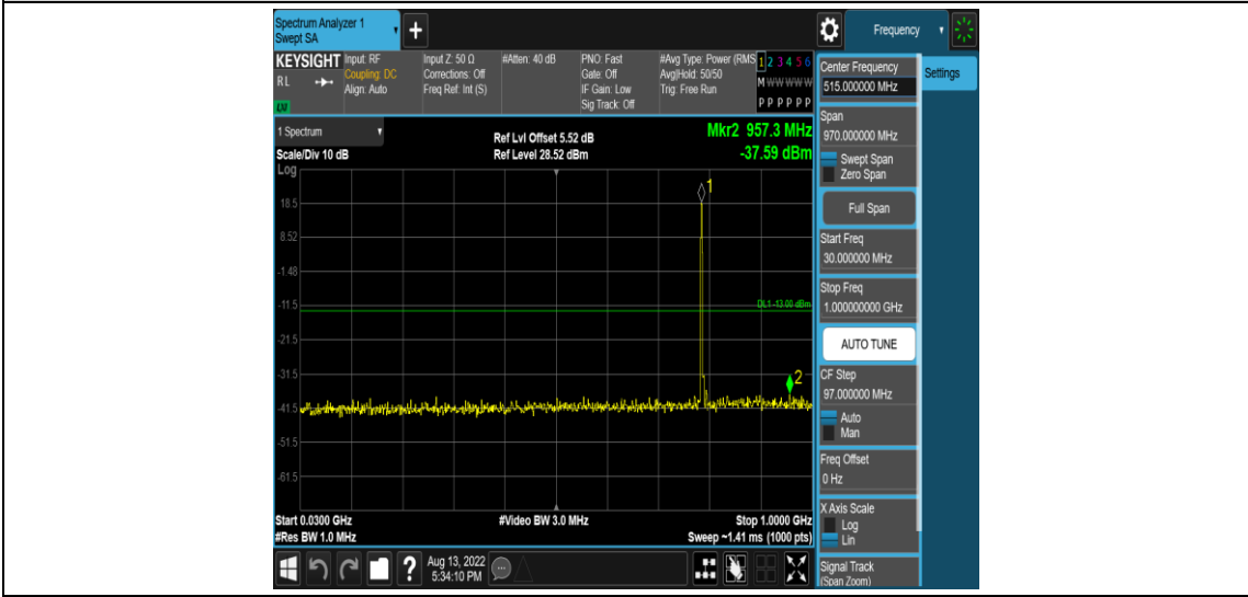
Band14-5MHz-QPSK-23330-1RB#0-Range3:30~1000MHz
