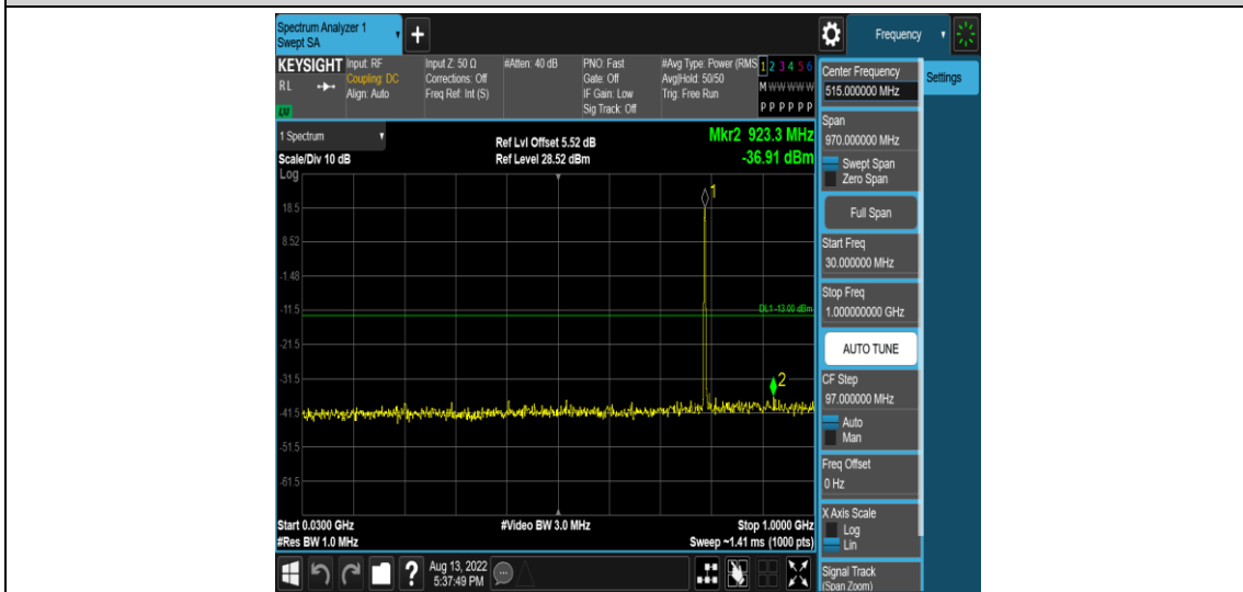
Band14-5MHz-QPSK-23355-1RB#0-Range3:30~1000MHz
