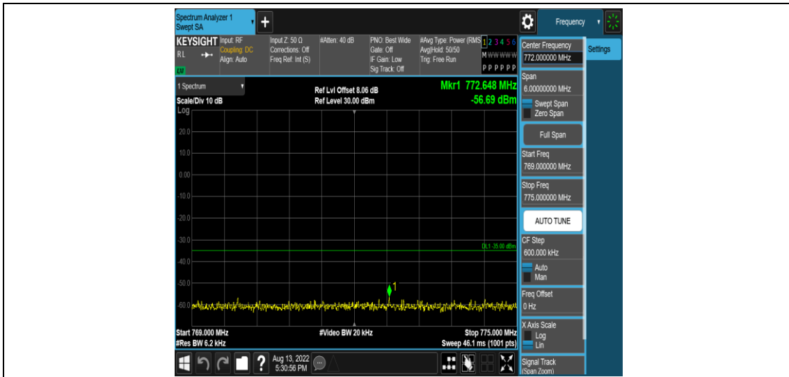
Band14-5MHz-QPSK-23305-1RB#0-Range5:769~775MHz
