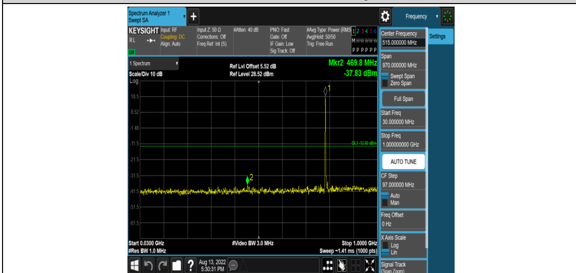
Band14-5MHz-QPSK-23305-1RB#0-Range3:30~1000MHz
