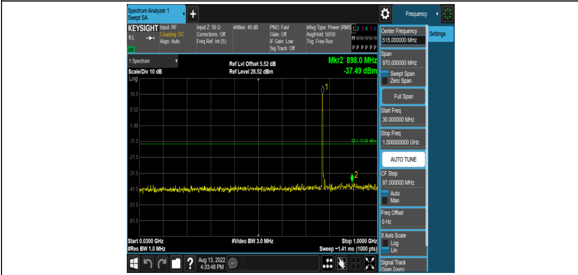
Band13-5MHz-16QAM-23205-1RB#0-Range3:30~1000MHz
