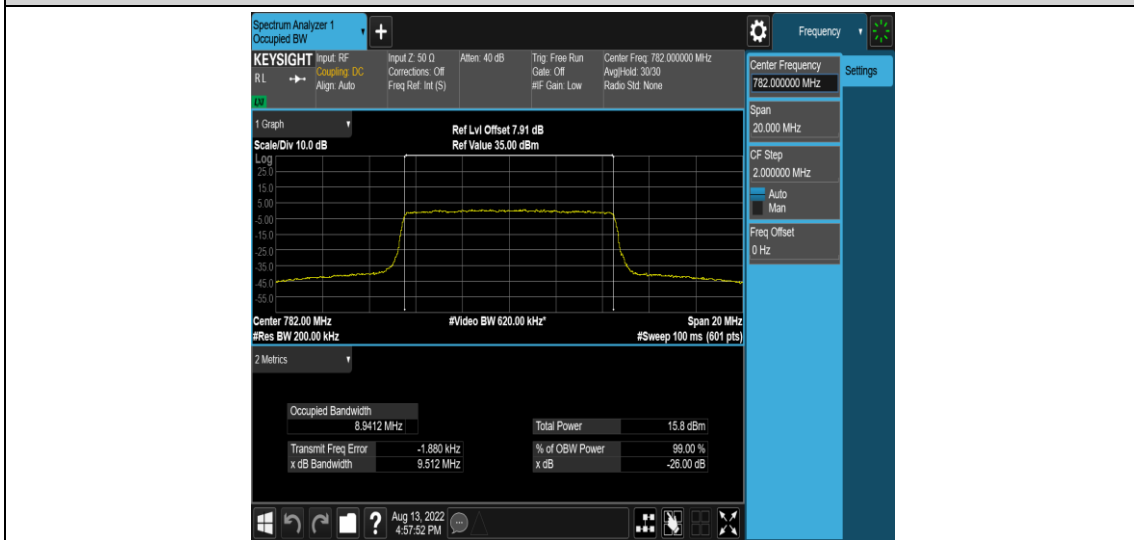
Band13-10MHz-16QAM-23230-50RB#0
