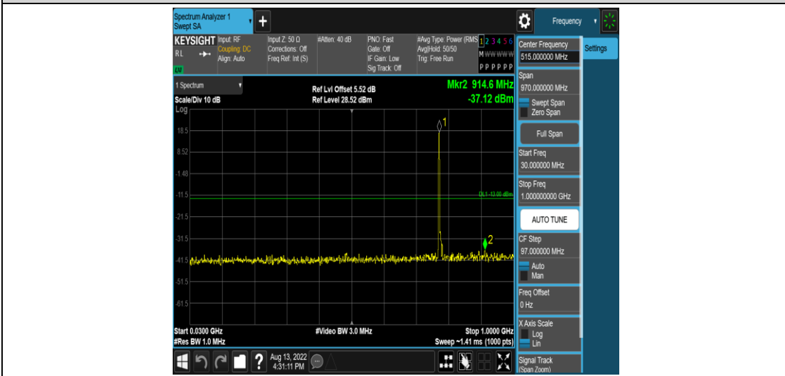
Band13-5MHz-QPSK-23205-1RB#0-Range3:30~1000MHz
