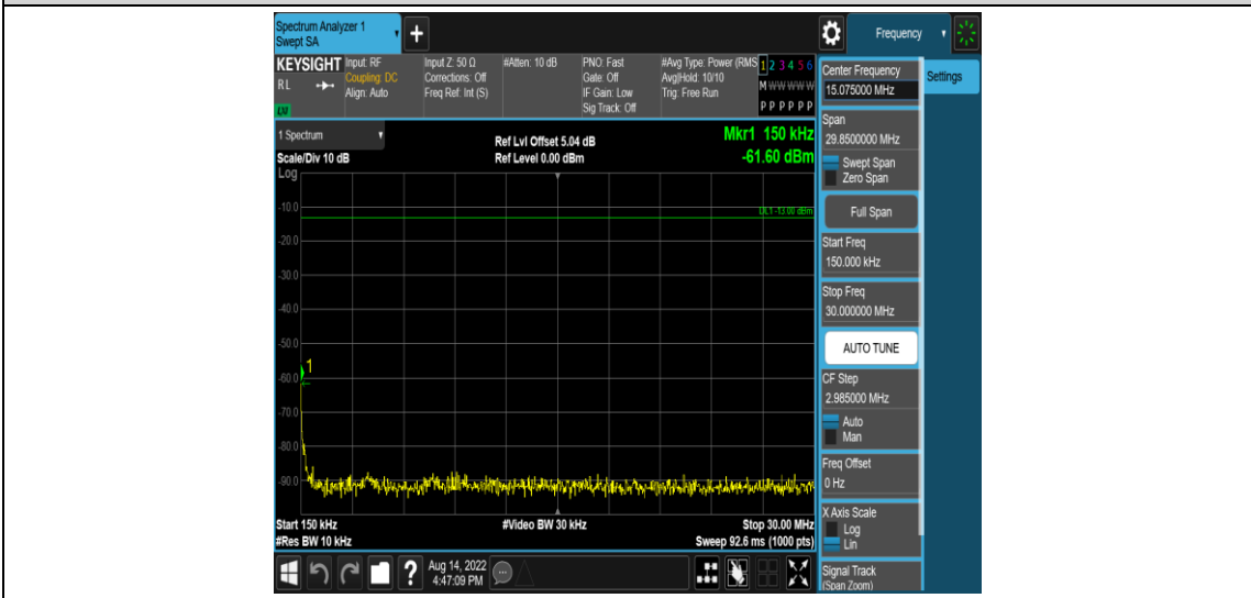
Band71-10MHz-16QAM-133297-1RB#0-Range2:0.15~30MHz
