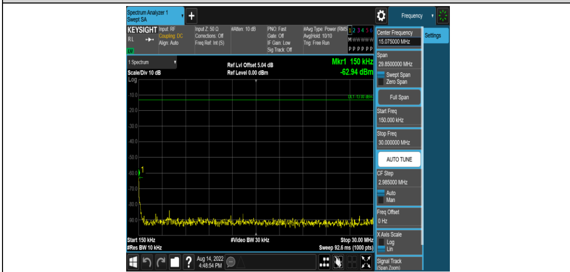
Band71-10MHz-16QAM-133422-1RB#0-Range2:0.15~30MHz
