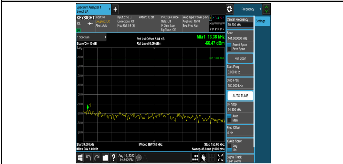
Band71-10MHz-16QAM-133422-1RB#0-Range1:0.009~0.15MHz
