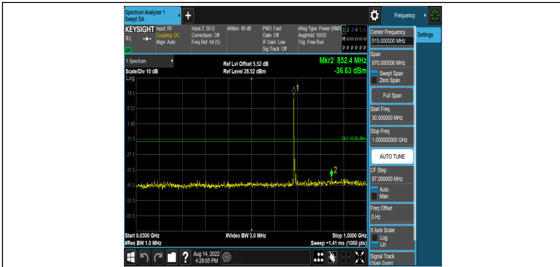
Band71-5MHz-16QAM-133447-1RB#0-Range3:30~1000MHz
