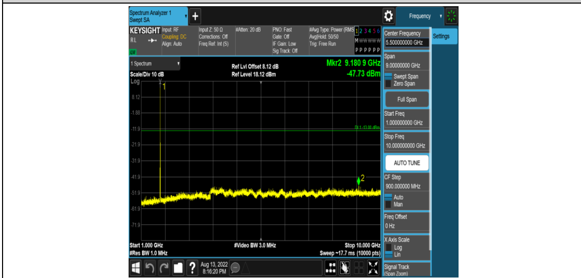
Band66-5MHz-16QAM-131997-1RB#0-Range4:1000~10000MHz
