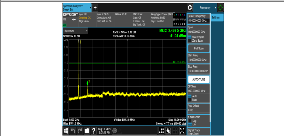
Band66-15MHz-QPSK-132597-1RB#0-Range4:1000~10000MHz
