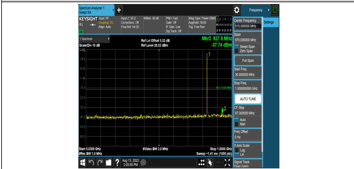
Band5-3MHz-QPSK-20525-1RB#0-Range3:30~1000MHz
