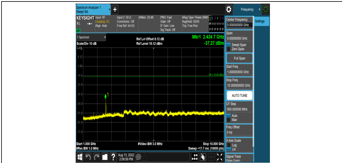
Band5-3MHz-16QAM-20525-1RB#0-Range4:1000~10000MHz
