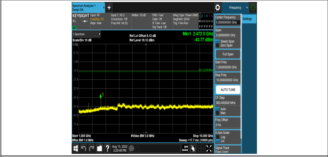
Band5-5MHz-QPSK-20425-1RB#0-Range4:1000~10000MHz
