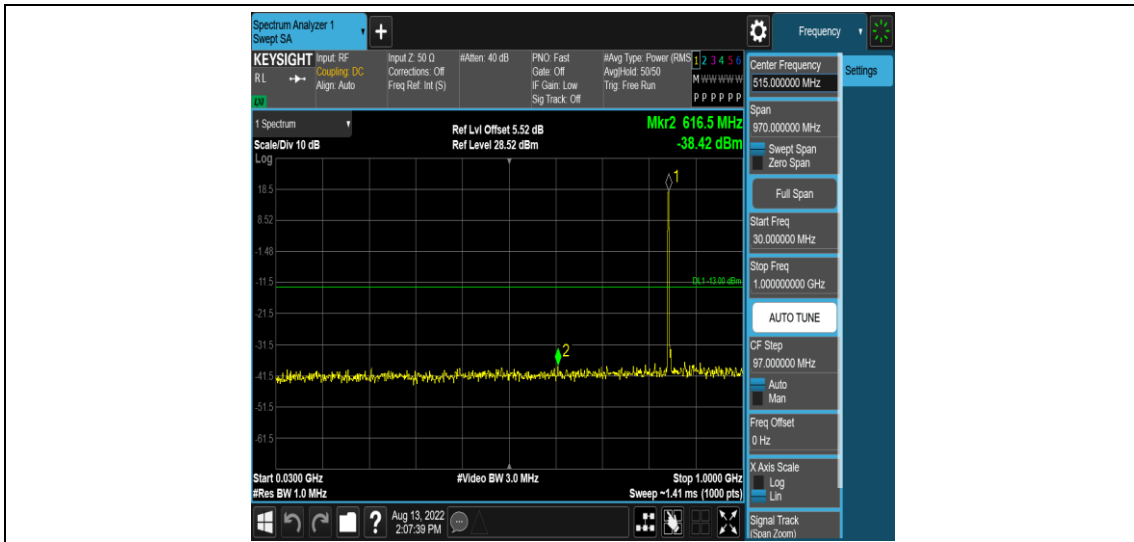
Band5-3MHz-QPSK-20635-1RB#0-Range3:30~1000MHz
