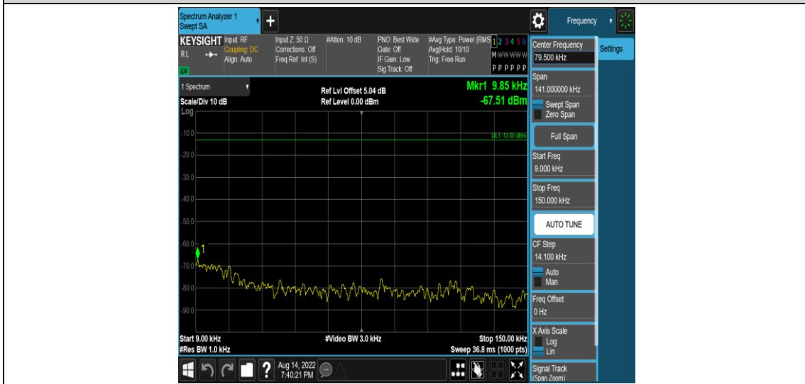
Band4-20MHz-QPSK-20175-1RB#0-Range1:0.009~0.15MHz
