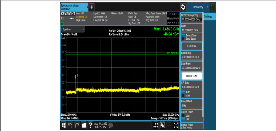
Band4-10MHz-16QAM-20175-1RB#0-Range5:2000~20000MHz
