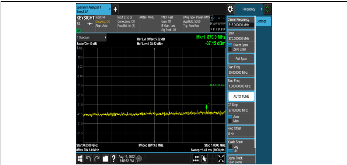
Band4-10MHz-16QAM-20175-1RB#0-Range3:30~1000MHz
