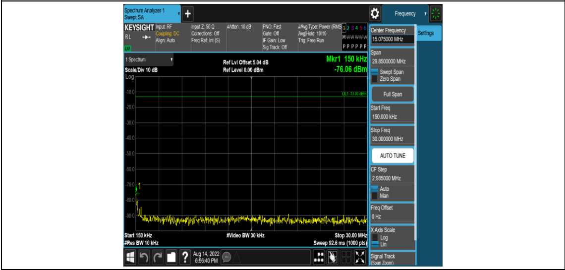
Band4-10MHz-16QAM-20175-1RB#0-Range2:0.15~30MHz
