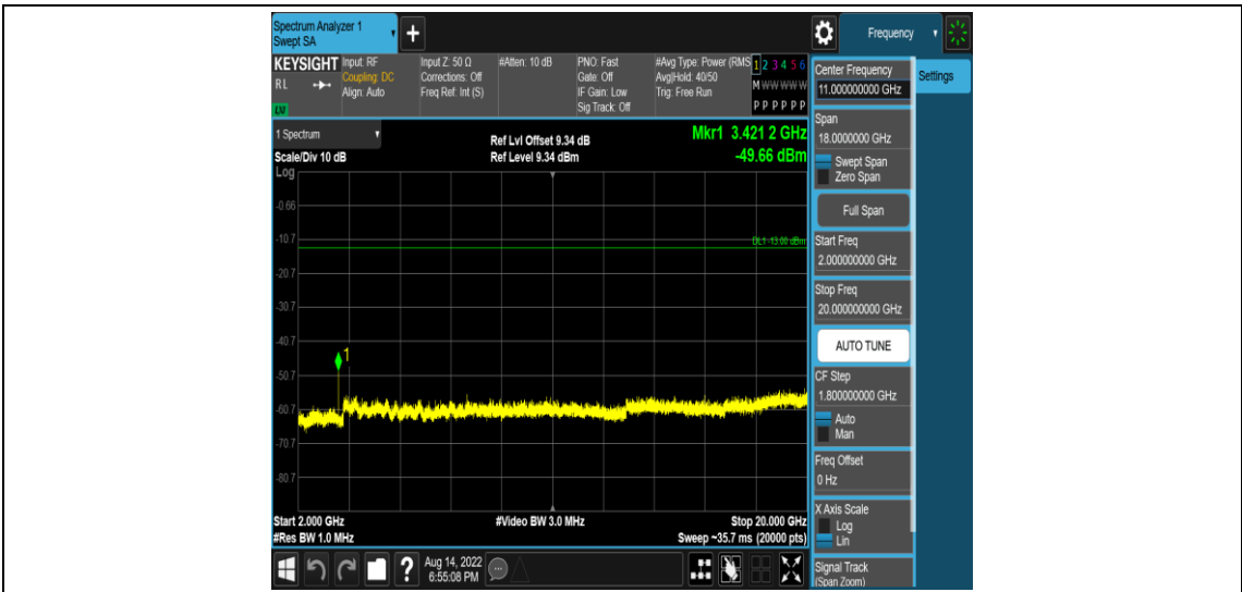
Band4-10MHz-16QAM-2000-1RB#0-Range5:2000~20000MHz
