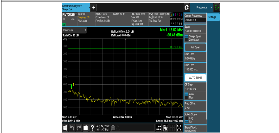
Band4-3MHz-16QAM-20175-1RB#0-Range1:0.009~0.15MHz
