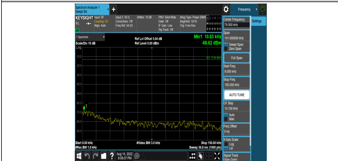
Band4-3MHz-16QAM-19965-1RB#0-Range1:0.009~0.15MHz
