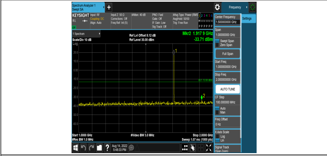
Band4-1.4MHz-16QAM-19957-1RB#0-Range4:1000~2000MHz
