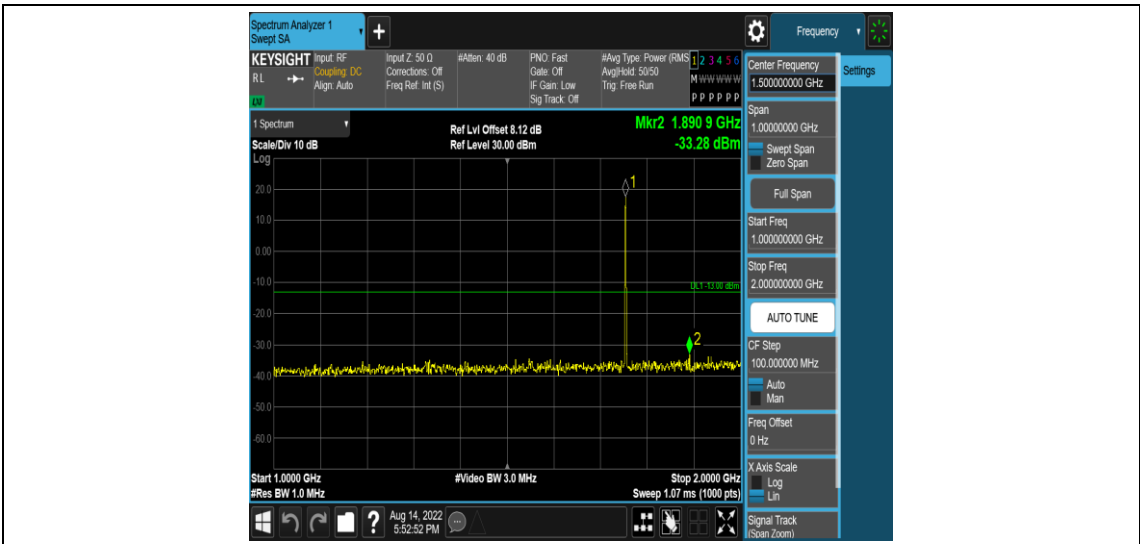
Band4-1.4MHz-16QAM-20393-1RB#0-Range4:1000~2000MHz
