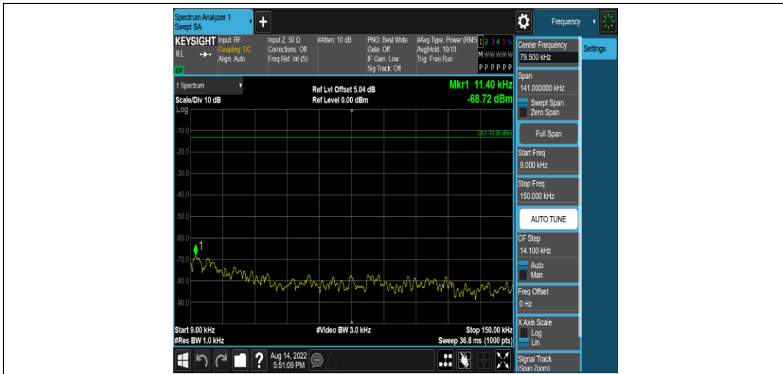
Band4-1.4MHz-QPSK-20393-1RB#0-Range1:0.009~0.15MHz
