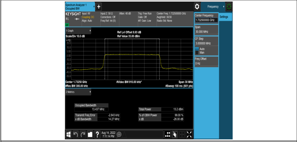
Band4-15MHz-16QAM-20175-75RB#0
