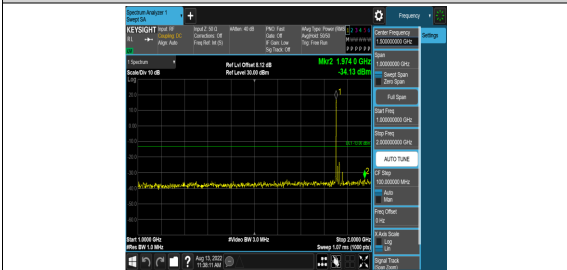
Band2-15MHz-QPSK-18675-1RB#0-Range4:1000~2000MHz
