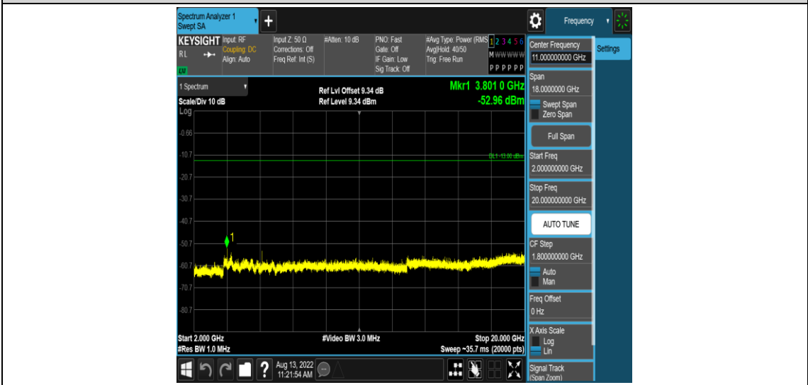
Band2-10MHz-16QAM-19150-1RB#0-Range5:2000~20000MHz
