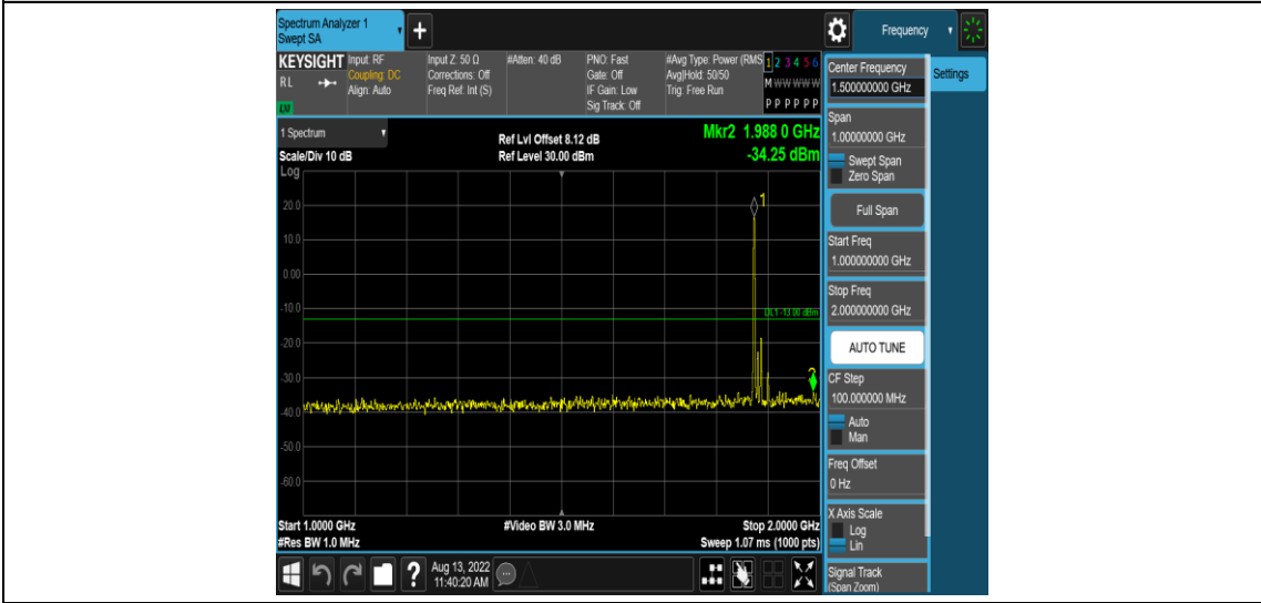
Band2-15MHz-QPSK-18900-1RB#0-Range4:1000~2000MHz
