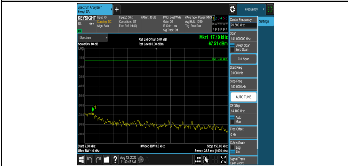
Band2-15MHz-16QAM-18900-1RB#0-Range1:0.009~0.15MHz
