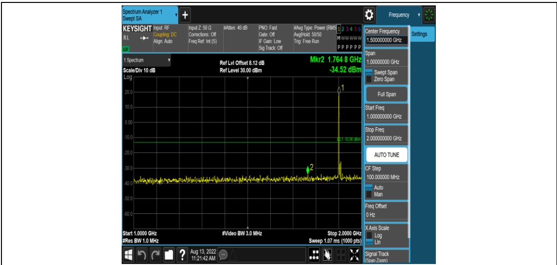
Band2-10MHz-16QAM-19150-1RB#0-Range4:1000~2000MHz
