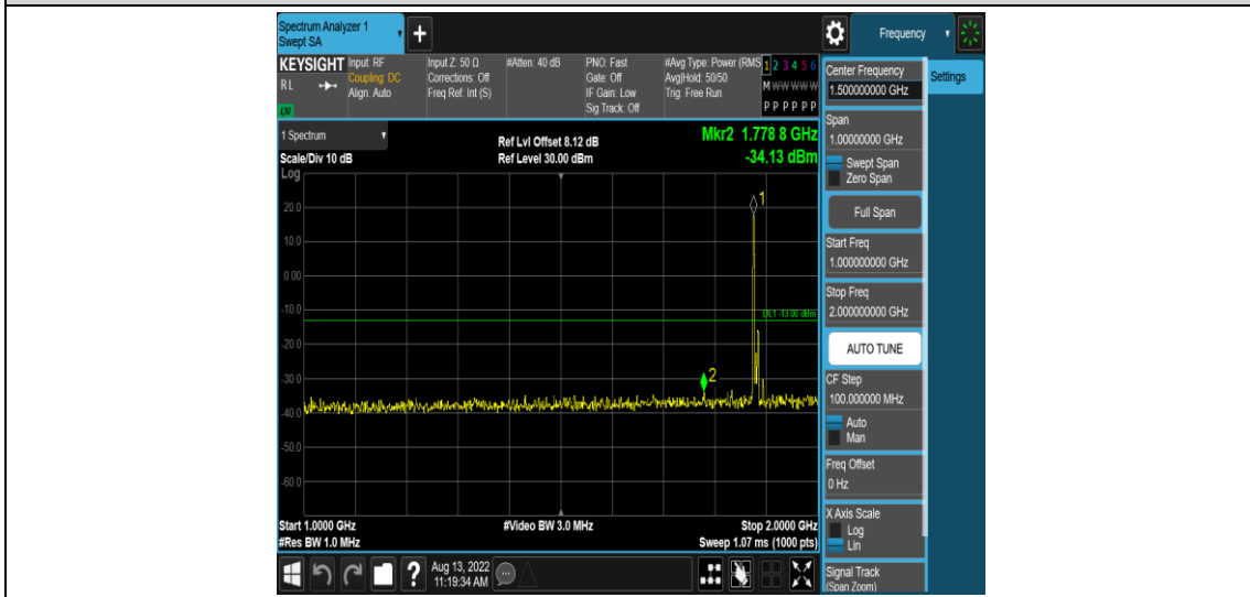
Band2-10MHz-16QAM-18900-1RB#0-Range4:1000~2000MHz
