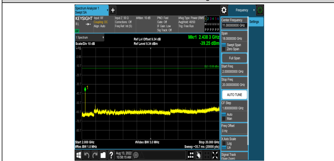
Band2-5MHz-16QAM-18900-1RB#0-Range5:2000~20000MHz
