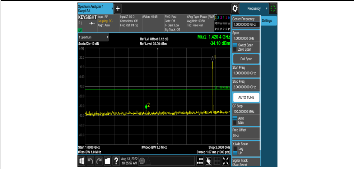
Band2-3MHz-16QAM-18900-1RB#0-Range4:1000~2000MHz
