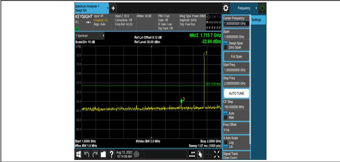
Band2-1.4MHz-16QAM-18900-1RB#0-Range4:1000~2000MHz
