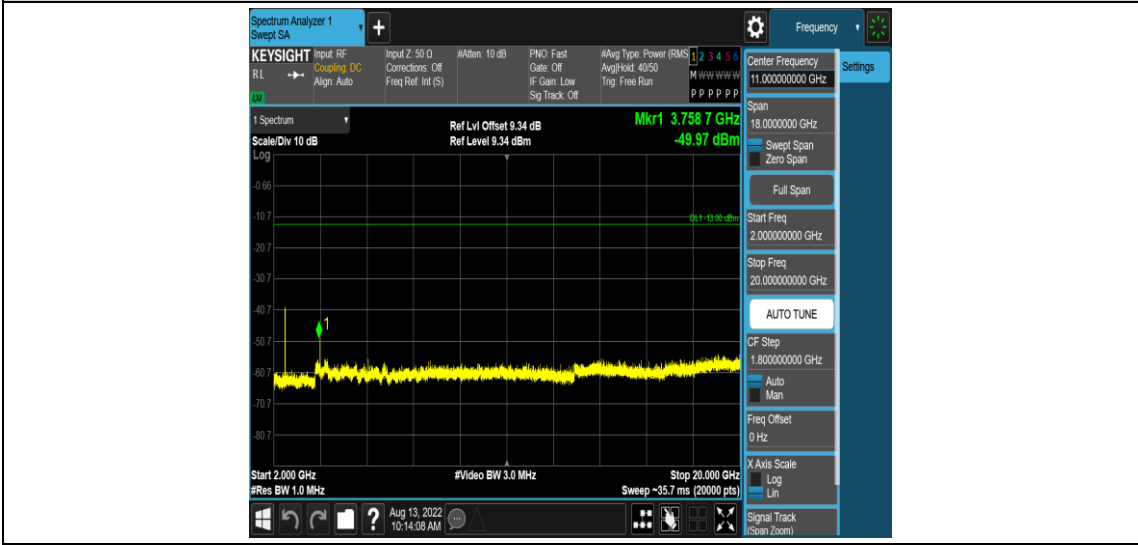
Band2-1.4MHz-QPSK-18900-1RB#0-Range5:2000~20000MHz
