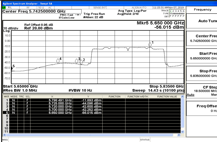
IEEE 802.11ac80 / Channel 155 / 5775MHz / Average
