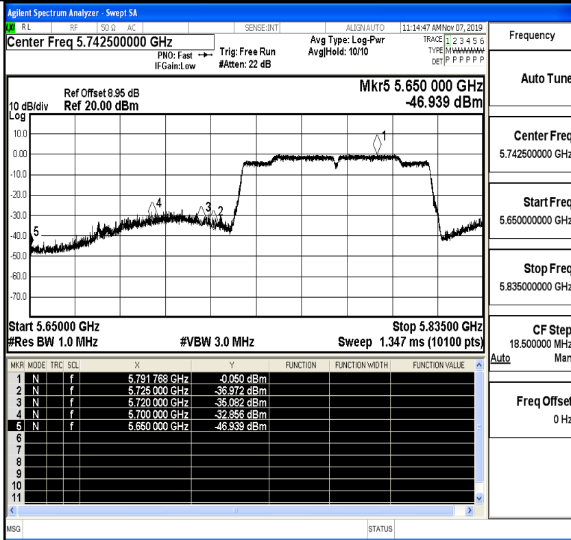
IEEE 802.11ac80 / Channel 155 / 5775MHz / Peak
