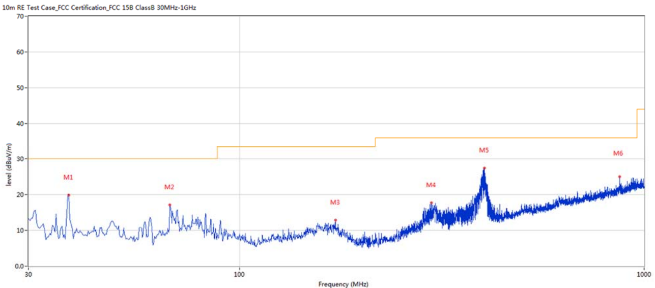
30 MHz to 1 GHz, ANT V
