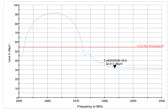
802.11b-Channel 11 Average
