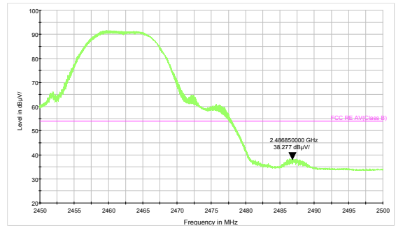
802.11g, Channel No.: 11 - PK
