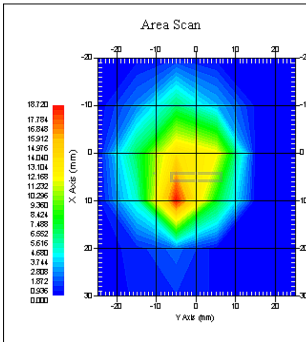
5800 MHz System Validation with Head tissue
