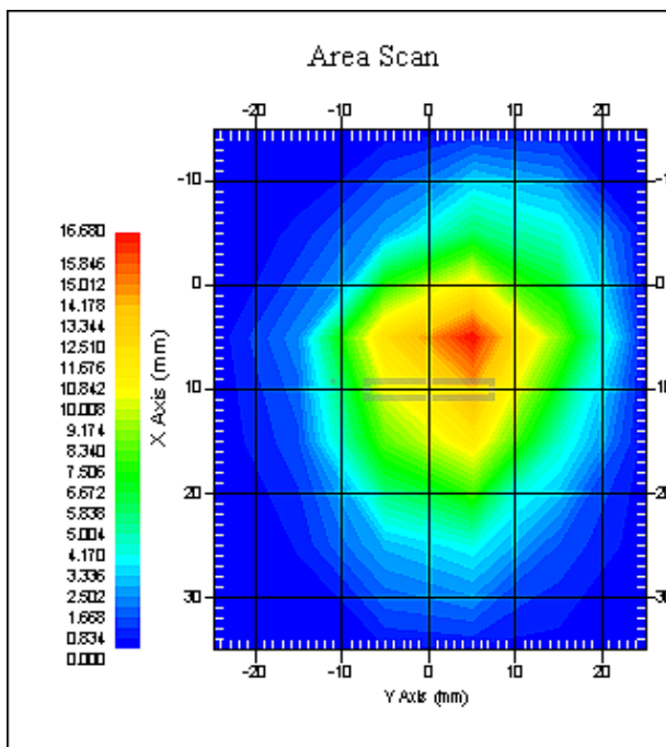
5250 MHz System Validation with Head tissue
