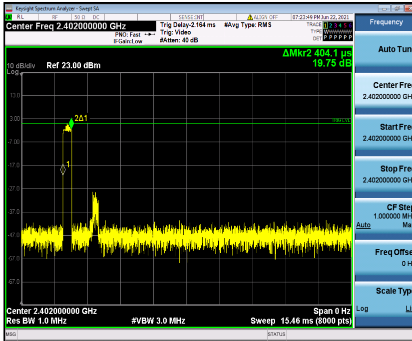
3DH1_Ant1_Hop_2402
