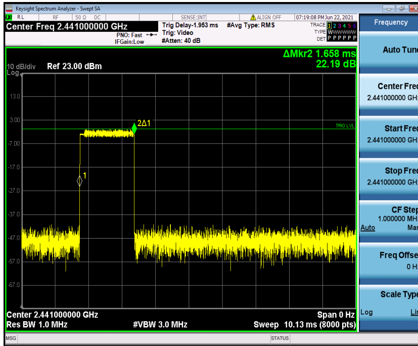
2DH3_Ant1_Hop_2441
