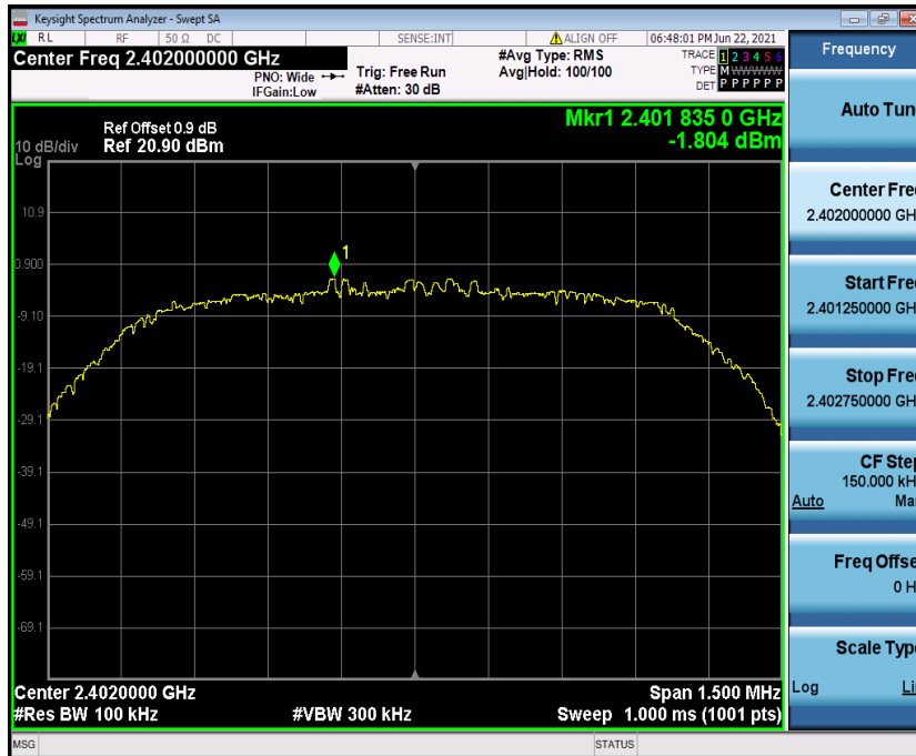
2DH5_Ant1_2402_0~Reference
