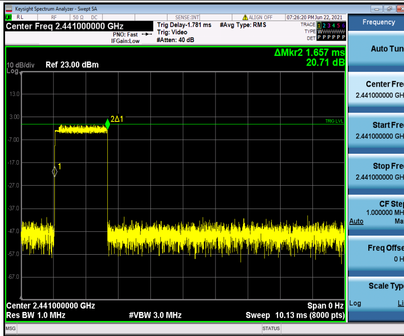
3DH3_Ant1_Hop_2441
