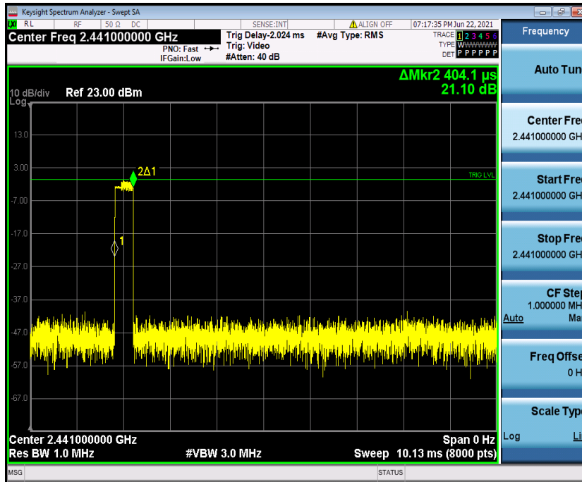
2DH1_Ant1_Hop_2441
