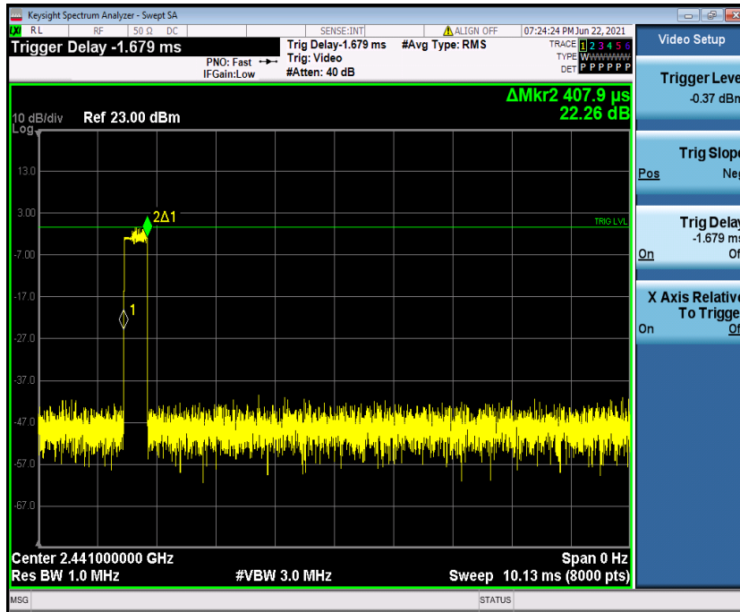
3DH1_Ant1_Hop_2441
