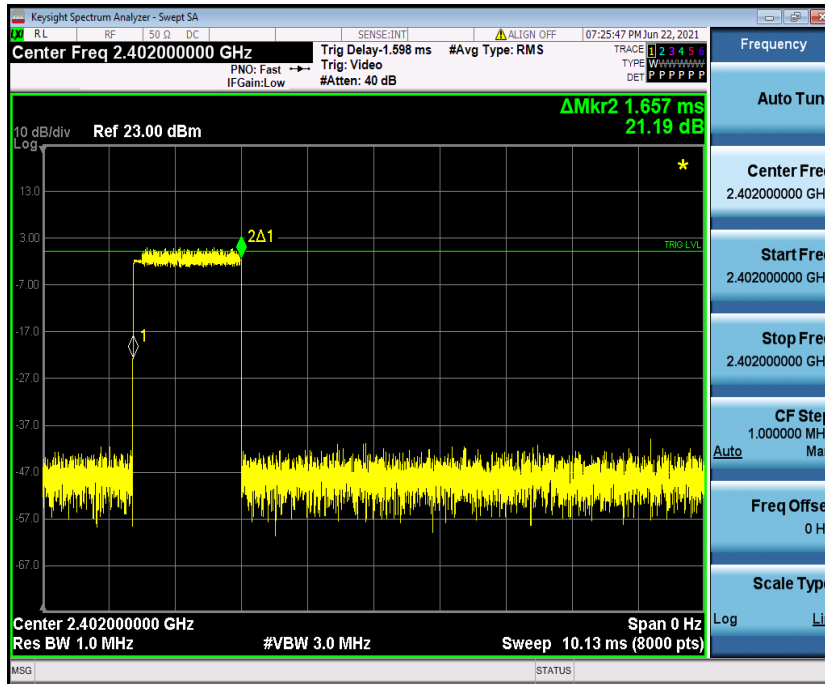
3DH3_Ant1_Hop_2402
