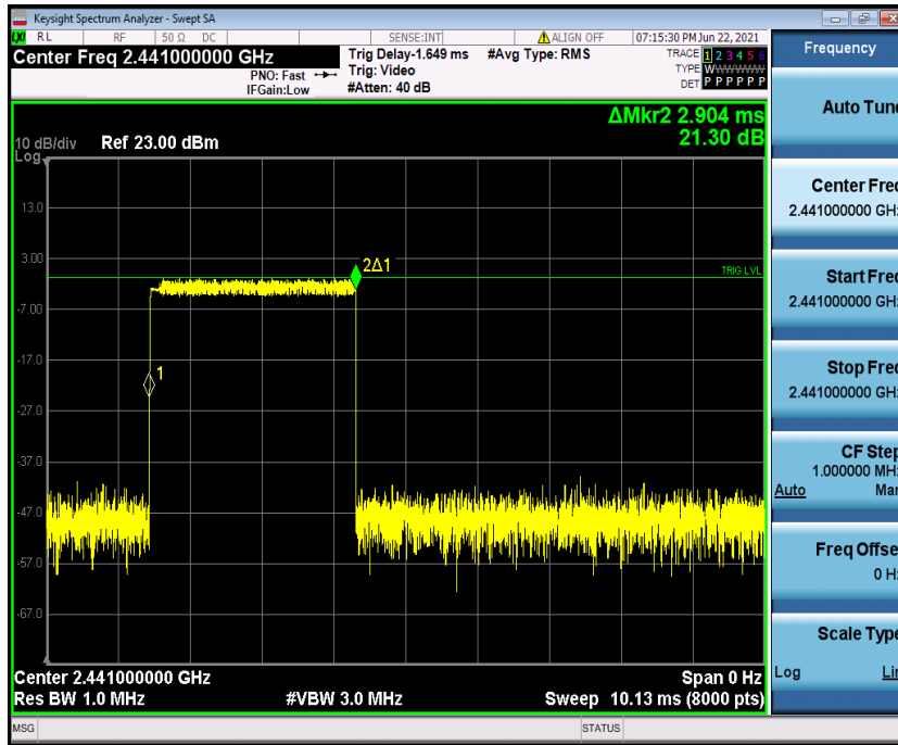
2DH5_Ant1_Hop_2441
