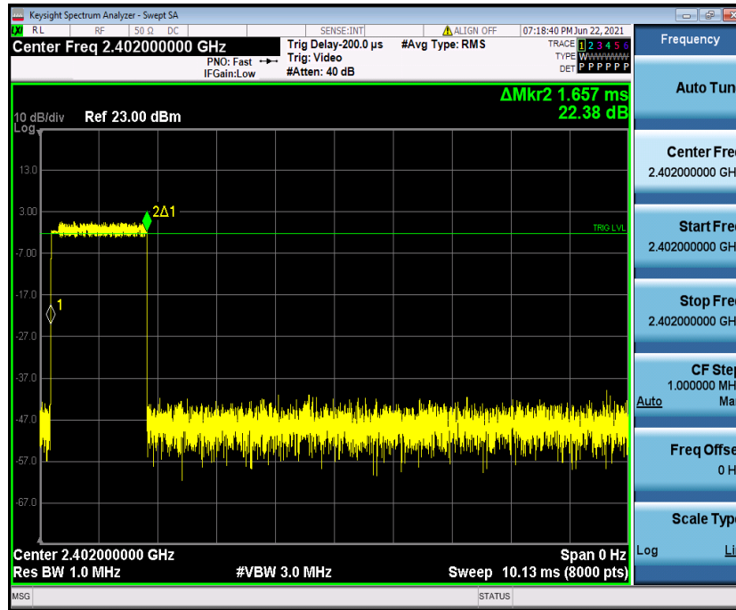
2DH3_Ant1_Hop_2402
