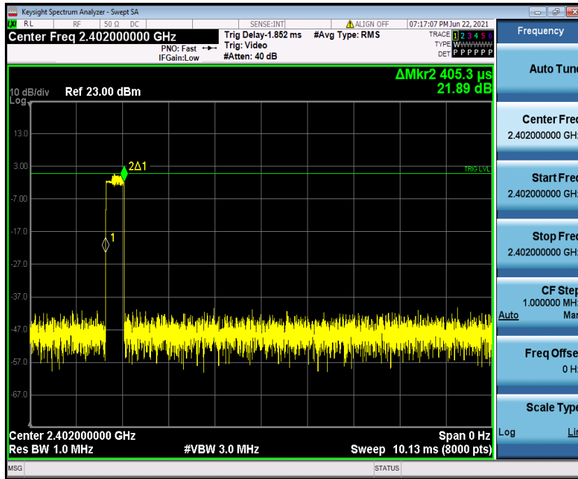
2DH1_Ant1_Hop_2402
