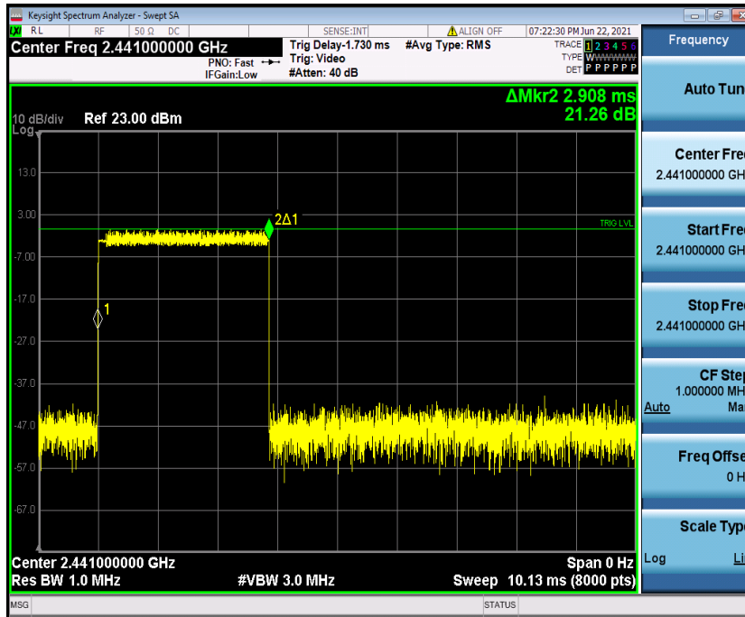
3DH5_Ant1_Hop_2441
