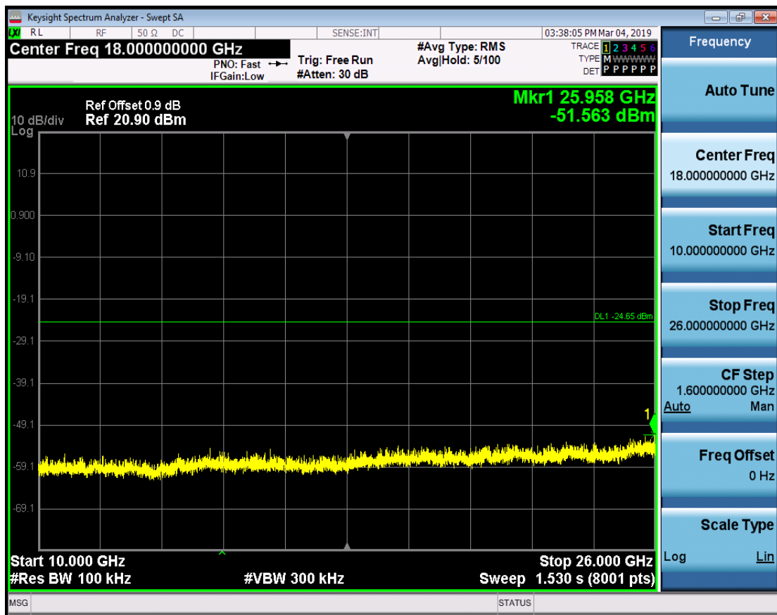
RF Conducted Spurious Emissions_2DH5_2441
