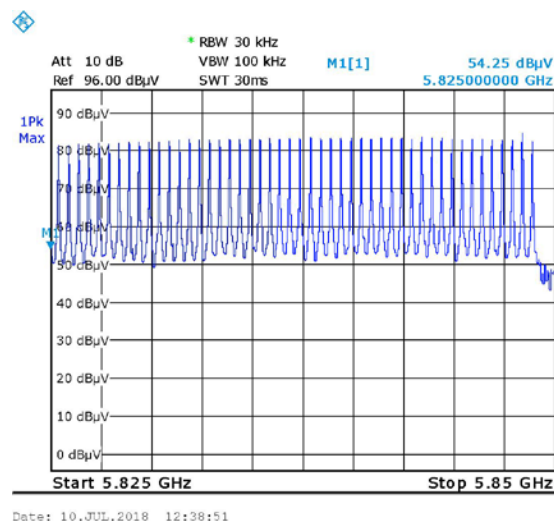
Figure 30. Number of Channels 5825-5850MHz band
