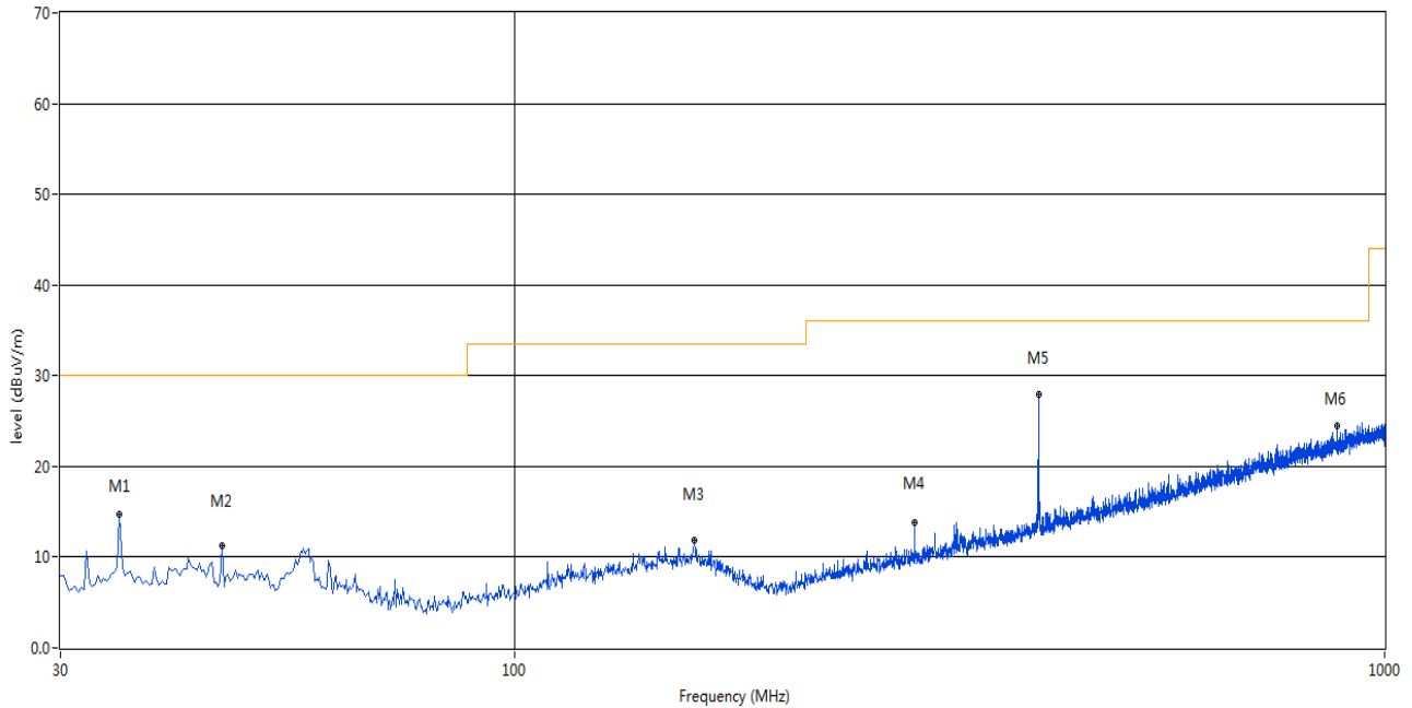
10m RE Test Case_FCC Certification_FCC 15B ClassB 30MHz-1GHz
