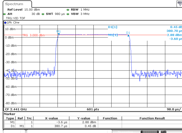
GFSK DH1
